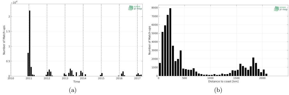
Figure 1: Number of match-ups between TSG-POLARSTERN and SMOS L3 v2 - Daily - 0.5 Deg (CATDS-CECOS-IFREMER) SSS as a function of time (a) and as function of the distance to coast (b) over the Southern Ocean Pi-MEP region and for the full satellite product period.
