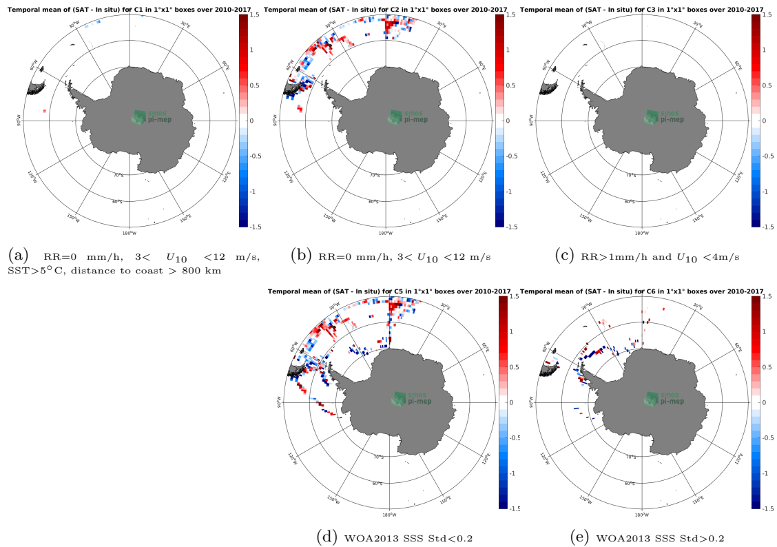
Figure 12: Temporal mean gridded over spatial boxes of size 1^{\circ}\times 1^{\circ} of \Delta\text{SSS} (SMOS L3 v2 - Daily - 0.5 Deg (CATDS-CECOS-IFREMER) - TSG-POLARSTERN) for 5 different subdatasets corresponding to:RR=0 mm/h, 3 < U_{10} < 12 m/s, SST >5^{\circ}\text{C} , distance to coast > 800 km (a), RR=0 mm/h, 3 < U_{10} < 12 m/s (b), RR >1 mm/h and U_{10} < 4 m/s (c), WOA2013 SSS Std <0.2 (d), WOA2013 SSS Std >0.2 (e).
