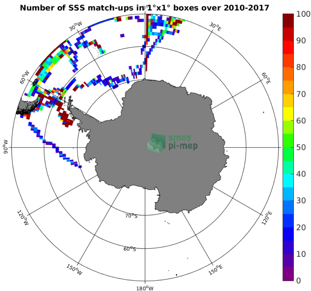
Figure 4: Number of SSS match-ups between TSG-POLARSTERN SSS and the SMOS L3 v2 - Daily - 0.5 Deg (CATDS-CECOS-IFREMER) SSS product for the Southern Ocean Pi-MEP region over 1^\circ \times 1^\circ boxes and for the full satellite product period.
