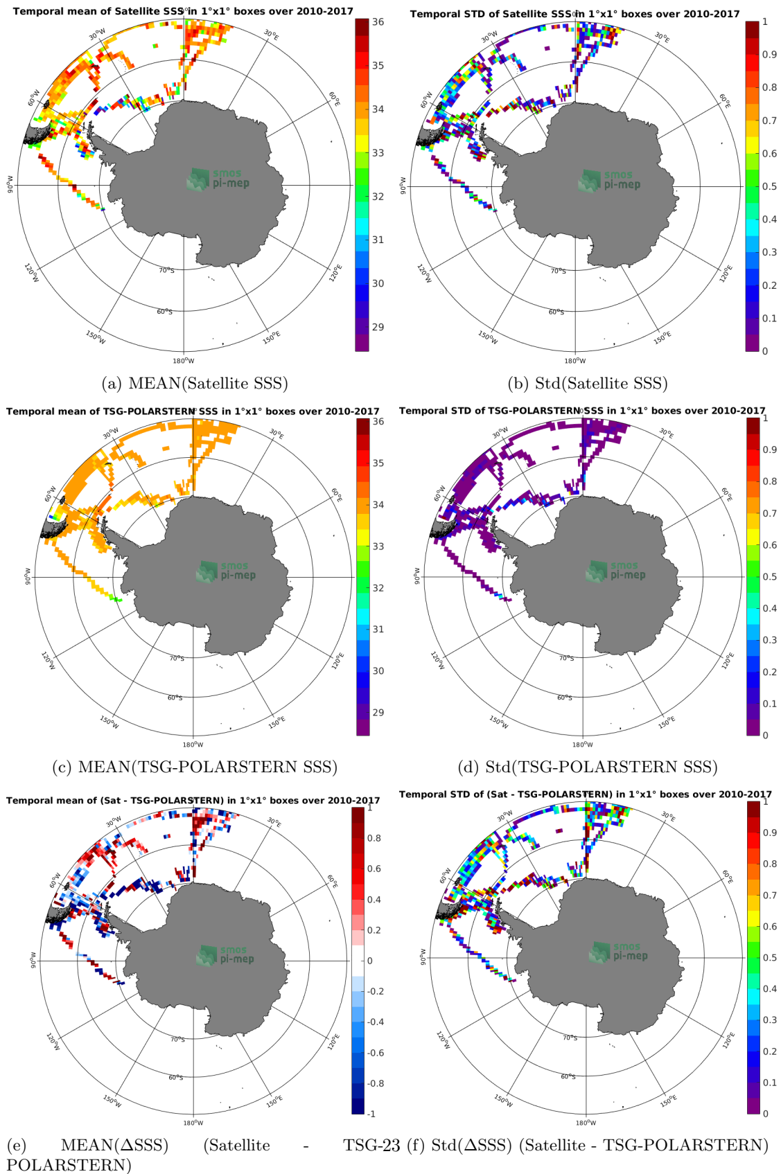
Figure 6: Temporal mean (left) and Std (right) of SSS from SMOS L3 v2 - Daily - 0.5 Deg (CATDS-CECOS-IFREMER) (top), TSG-POLARSTERN (middle), and of \Delta SSS (Satellite - TSG-POLARSTERN). Only match-up pairs are used to generate these maps.
