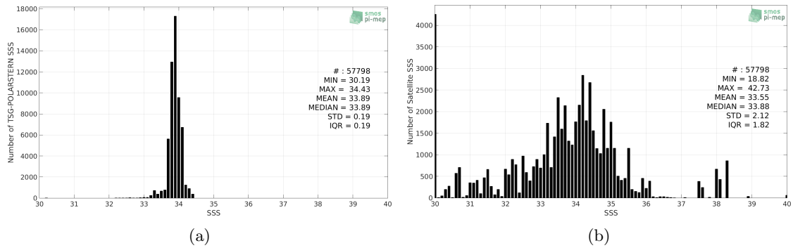
Figure 2: Histograms of SSS from TSG-POLARSTERN (a) and SMOS L3 v2 - Daily - 0.5 Deg (CATDS-CECOS-IFREMER) (b) considering all match-up pairs per bins of 0.1 over the Southern Ocean Pi-MEP region and for the full satellite product period.
