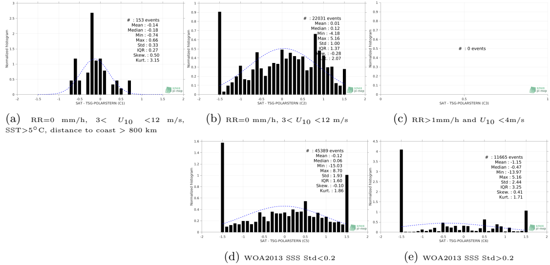
Figure 13: Normalized histogram of \Delta SSS (SMOS L3 v2 - Daily - 0.5 Deg (CATDS-CECOS-IFREMER) - TSG-POLARSTERN) for 5 different subdatasets corresponding to: RR=0 mm/h, 3 < U_{10} < 12 m/s, SST > 5°C, distance to coast > 800 km (a), RR=0 mm/h, 3 < U_{10} < 12 m/s (b), RR > 1mm/h and U_{10} < 4 m/s (c), WOA2013 SSS Std < 0.2 (d), WOA2013 SSS Std > 0.2 (e).
