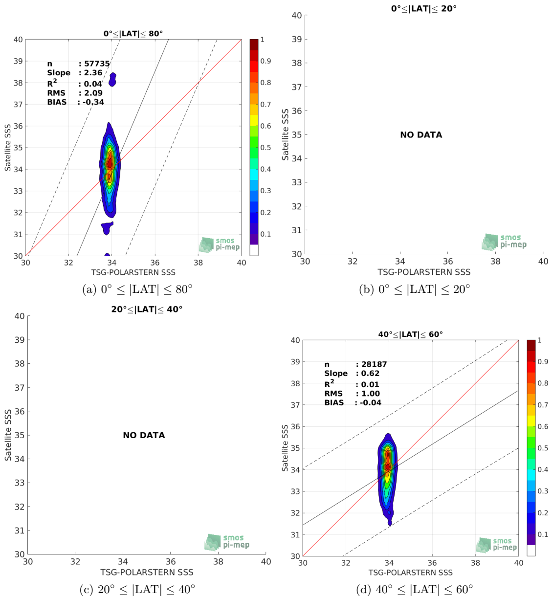
Figure 9: Contour maps of the concentration of SMOS L3 v2 - Daily - 0.5 Deg (CATDS-CECOS-IFREMER) SSS (y-axis) versus TSG-POLARSTERN SSS (x-axis) at match-up pairs for different latitude bands. For each plot, the red line shows x=y . The black thin and dashed lines indicate a linear fit through the data cloud and the \pm 95\% confidence levels, respectively. The number match-up pairs n , the slope and R^2 coefficient of the linear fit, the root mean square (RMS) and the mean bias between satellite and in situ data are indicated for each latitude band in each plots.
