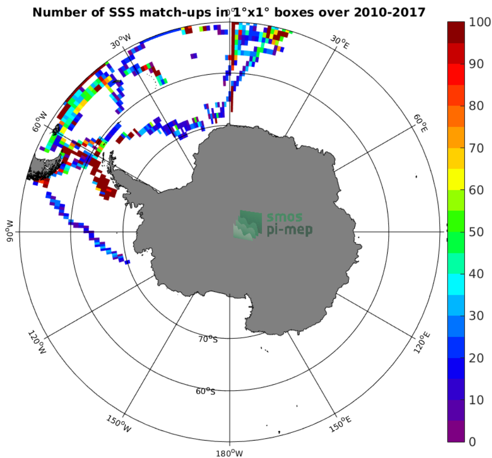
Figure 4: Number of SSS match-ups between TSG-POLARSTERN SSS and the SMOS-L3-CATDS-CECOS-IFREMER-V2-1DAY-0.5DEG SSS product for the Southern Ocean Pi-MEP region over 1^\circ \times 1^\circ boxes and for the full satellite product period.
