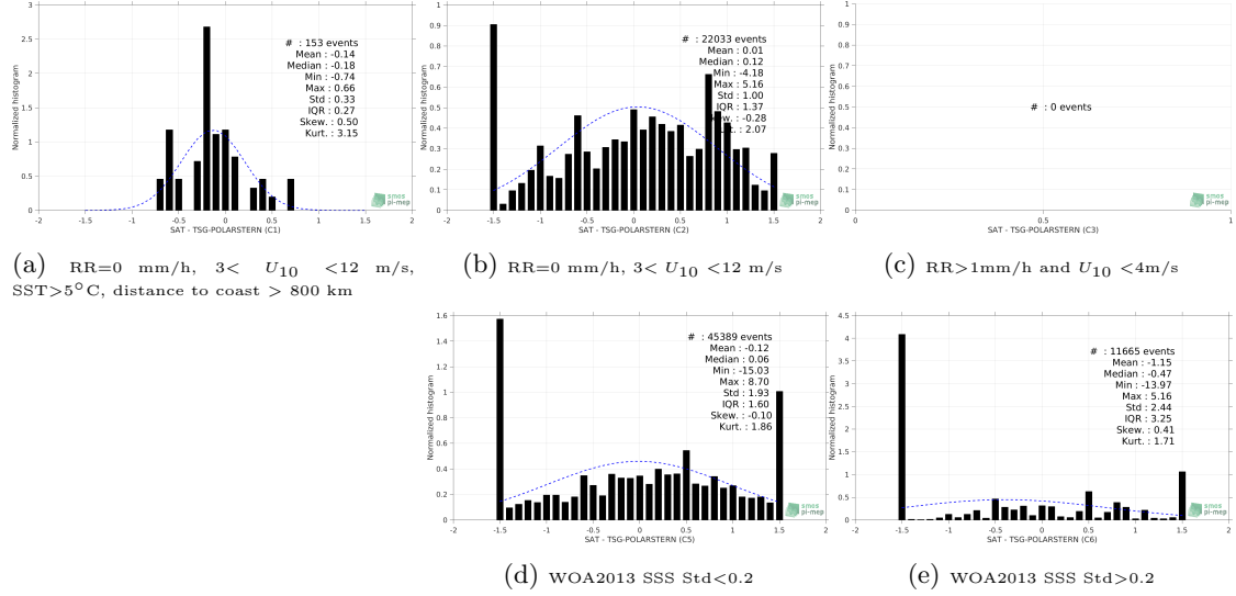
Figure 13: Normalized histogram of \Delta SSS (SMOS-L3-CATDS-CECOS-IFREMER-V2-1DAY-0.5DEG - TSG-POLARSTERN) for 5 different subdatasets corresponding to: RR=0 mm/h, 3 < U_{10} < 12 m/s, SST > 5°C, distance to coast > 800 km (a), RR=0 mm/h, 3 < U_{10} < 12 m/s (b), RR > 1mm/h and U_{10} < 4 m/s (c), WOA2013 SSS Std < 0.2 (d), WOA2013 SSS Std > 0.2 (e).
