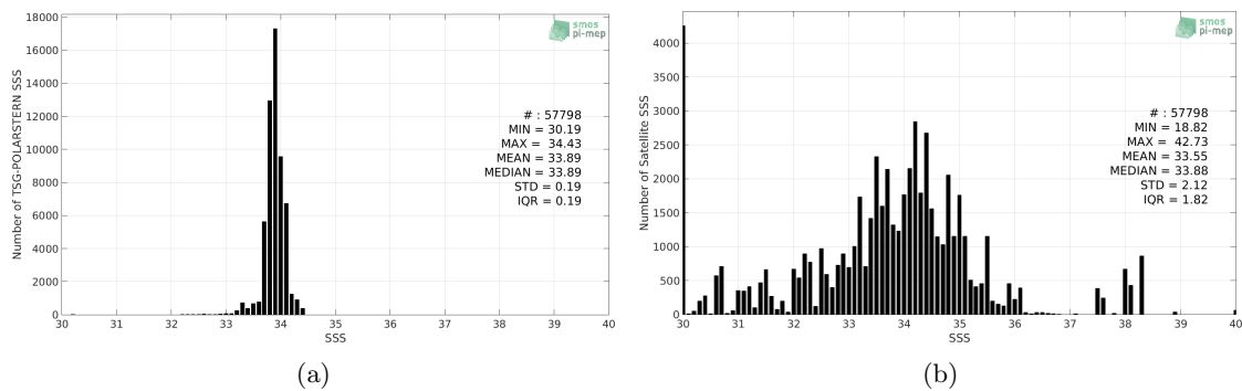
Figure 2: Histograms of SSS from TSG-POLARSTERN (a) and SMOS-L3-CATDS-CECOS-IFREMER-V2-1DAY-0.5DEG (b) considering all match-up pairs per bins of 0.1 over the Southern Ocean Pi-MEP region and for the full satellite product period.
