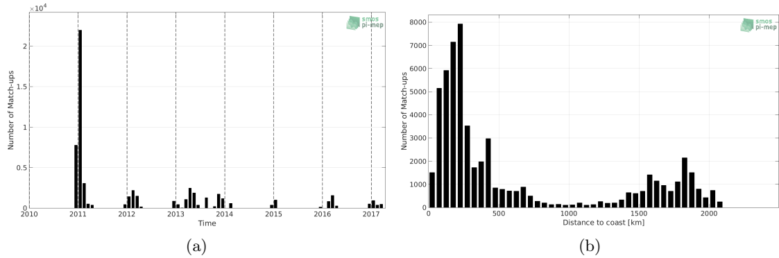
Figure 1: Number of match-ups between TSG-POLARSTERN and SMOS-L3-CATDS-CECOS-IFREMER-V2-1DAY-0.5DEG SSS as a function of time (a) and as function of the distance to coast (b) over the Southern Ocean Pi-MEP region and for the full satellite product period.
