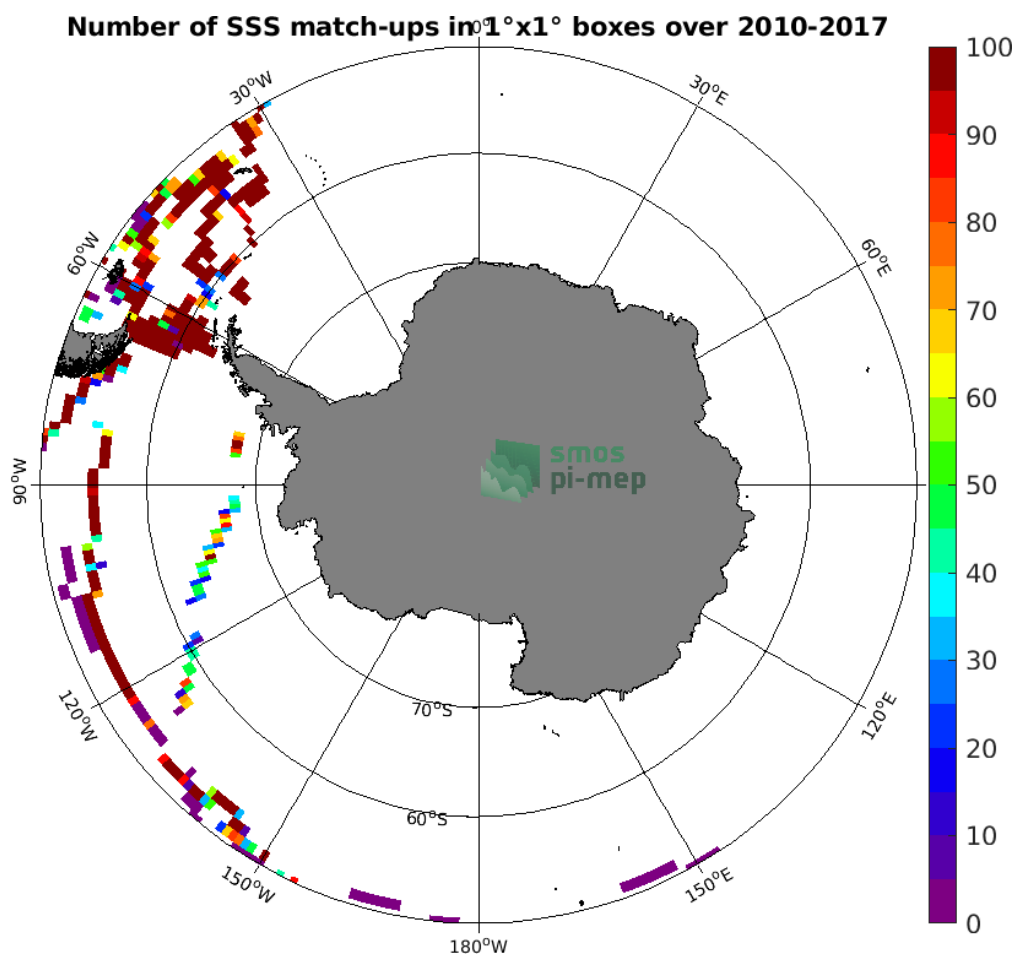
Figure 4: Number of SSS match-ups between TSG (GOSUD-Sailing-ship) SSS and the SMOS SSS L3 v2 - Daily - 0.5 Deg (CATDS-CECOS-IFREMER) SSS product for the Southern Ocean Pi-MEP region over 1^\circ \times 1^\circ boxes and for the full satellite product period.
