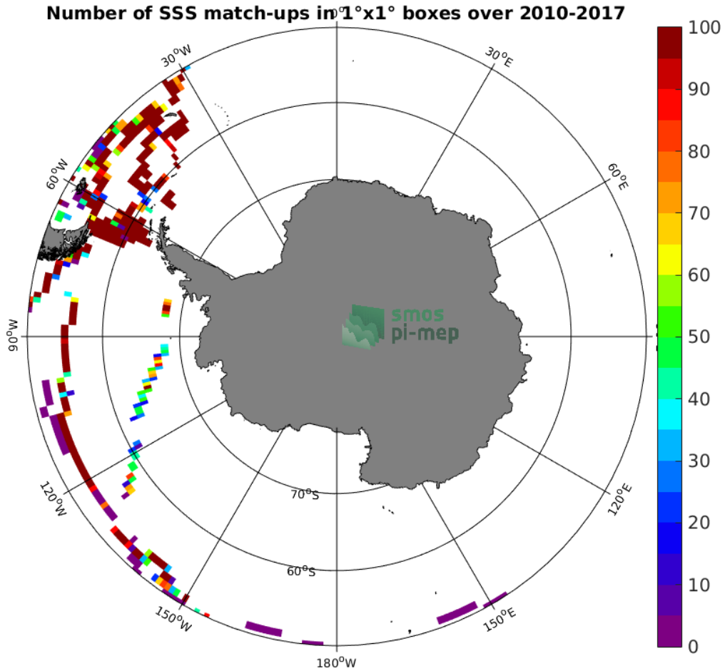
Figure 4: Number of SSS match-ups between TSG (GOSUD-Sailing-ship) SSS and the SMOS SSS L3 v2 - Daily - 0.5 Deg (CATDS-CECOS-IFREMER) SSS product for the Southern Ocean Pi-MEP region over 1°x1° boxes and for the full satellite product period.
