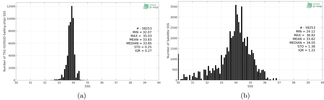
Figure 2: Histograms of SSS from TSG (GOSUD-Sailing-ship) (a) and SMOS SSS L3 v2 - Daily - 0.5 Deg (CATDS-CECOS-IFREMER) (b) considering all match-up pairs per bins of 0.1 over the Southern Ocean Pi-MEP region and for the full satellite product period.
