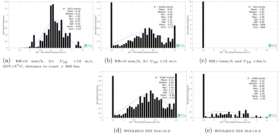
Figure 13: Normalized histogram of \Delta SSS (SMOS-L3-CATDS-CECOS-IFREMER-V2-1DAY-0.5DEG - TSG-GOSUD-Sailing-ship) for 5 different subdatasets corresponding to: RR=0 mm/h, 3 < U_{10} < 12 m/s, SST > 5°C, distance to coast > 800 km (a), RR=0 mm/h, 3 < U_{10} < 12 m/s (b), RR > 1mm/h and U_{10} < 4 m/s (c), WOA2013 SSS Std < 0.2 (d), WOA2013 SSS Std > 0.2 (e).
