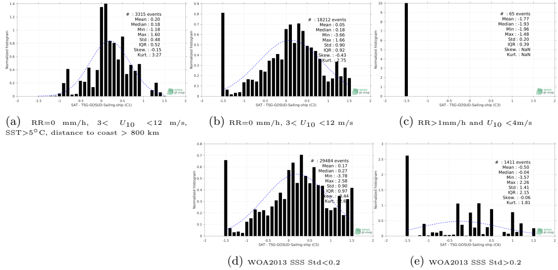
Figure 13: Normalized histogram of \Delta\text{SSS} (SMOS-L3-CATDS-CECOS-IFREMER-V2-1DAY-0.5DEG - TSG-GOSUD-Sailing-ship) for 5 different subdatasets corresponding to: RR=0 mm/h, 3 < U_{10} < 12 m/s, SST > 5^{\circ}\text{C} , distance to coast > 800 km (a), RR=0 mm/h, 3 < U_{10} < 12 m/s (b), RR > 1\text{mm/h} and U_{10} < 4\text{m/s} (c), WOA2013 SSS \text{Std} < 0.2 (d), WOA2013 SSS \text{Std} > 0.2 (e).
