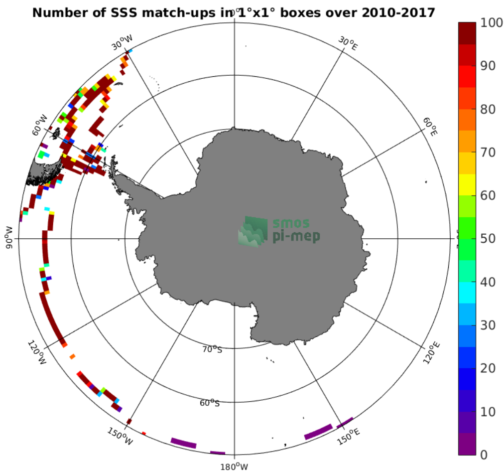
Figure 4: Number of SSS match-ups between TSG-GOSUD-Sailing-ship SSS and the SMOS-L3-CATDS-CECOS-IFREMER-V2-1DAY-0.5DEG SSS product for the Southern Ocean Pi-MEP region over 1°x1° boxes and for the full satellite product period.
