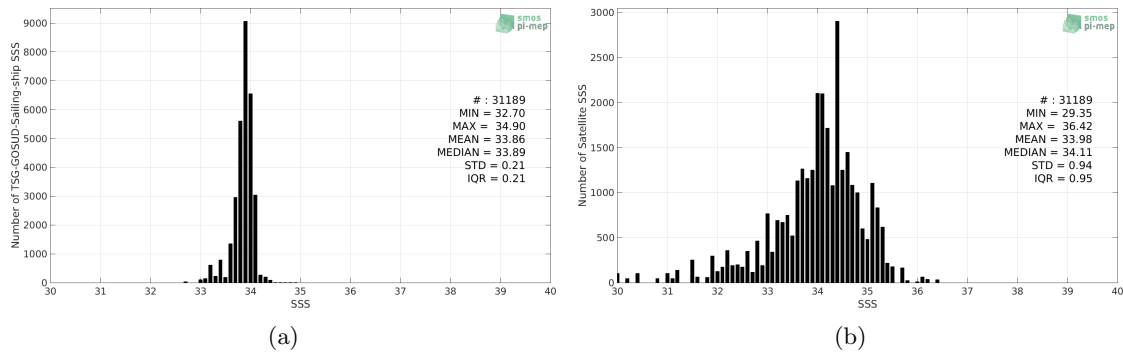
Figure 2: Histograms of SSS from TSG-GOSUD-Sailing-ship (a) and SMOS-L3-CATDS-CECOS-IFREMER-V2-1DAY-0.5DEG (b) considering all match-up pairs per bins of 0.1 over the Southern Ocean Pi-MEP region and for the full satellite product period.
