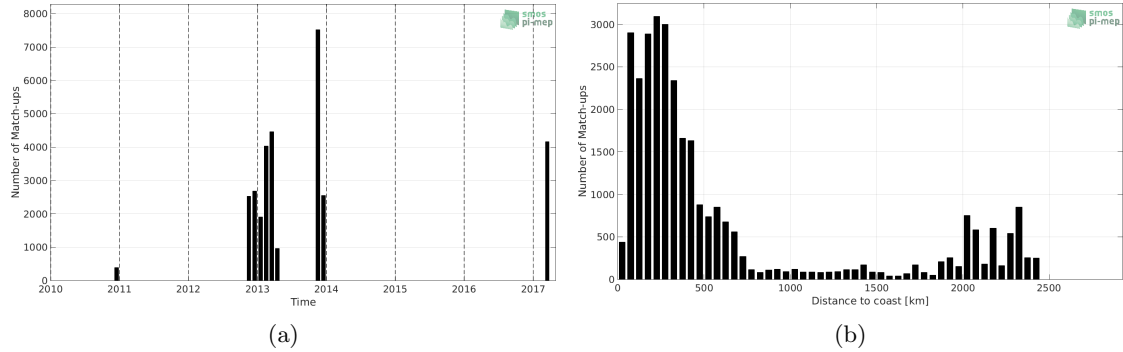
Figure 1: Number of match-ups between TSG-GOSUD-Sailing-ship and SMOS-L3-CATDS-CECOS-IFREMER-V2-1DAY-0.5DEG SSS as a function of time (a) and as function of the distance to coast (b) over the Southern Ocean Pi-MEP region and for the full satellite product period.
