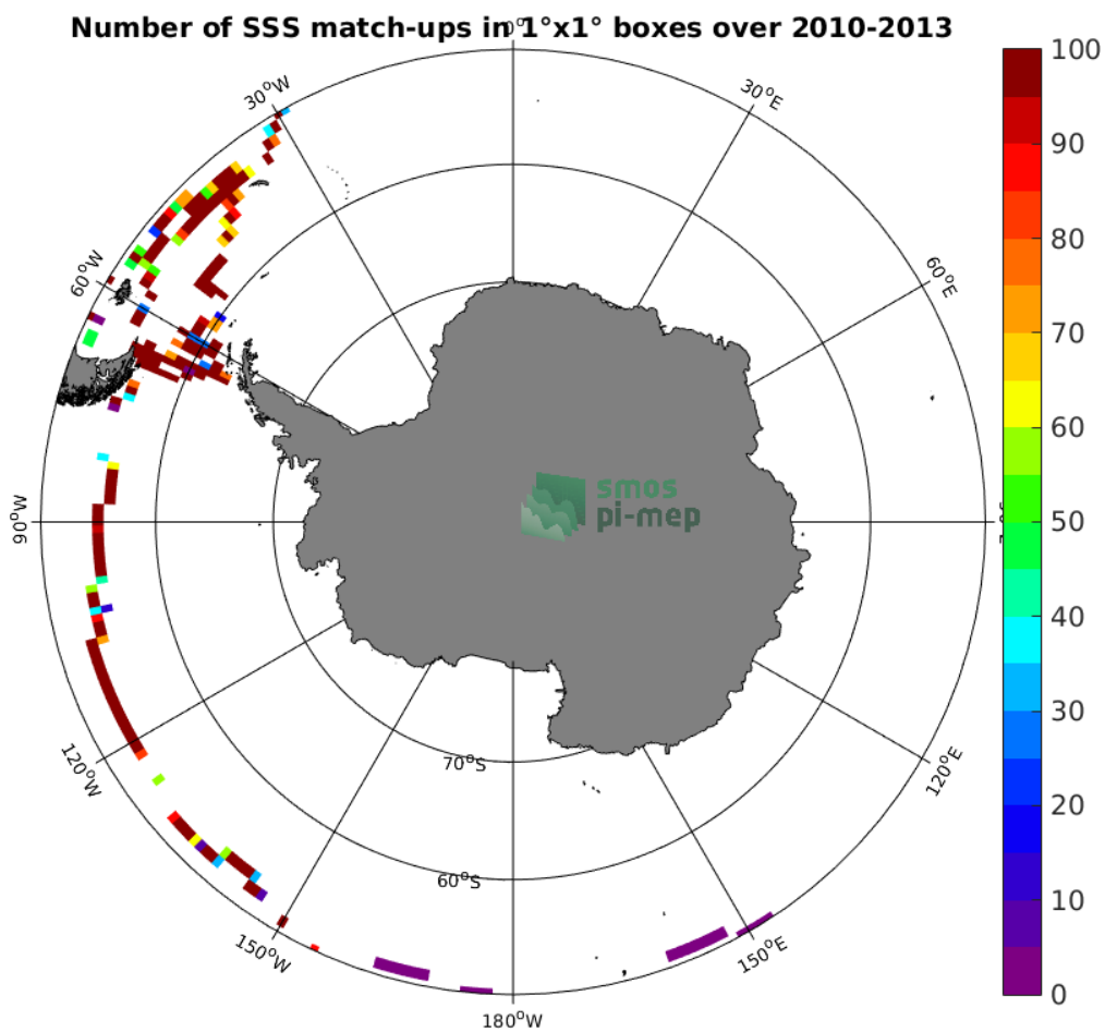
Figure 4: Number of SSS match-ups between TSG-GOSUD-Sailing-ship SSS and the SMOS-L3-CATDS-CECOS-IFREMER-V2-1DAY-0.5DEG SSS product for the Southern Ocean Pi-MEP region over 1^\circ \times 1^\circ boxes and for the full satellite product period.
