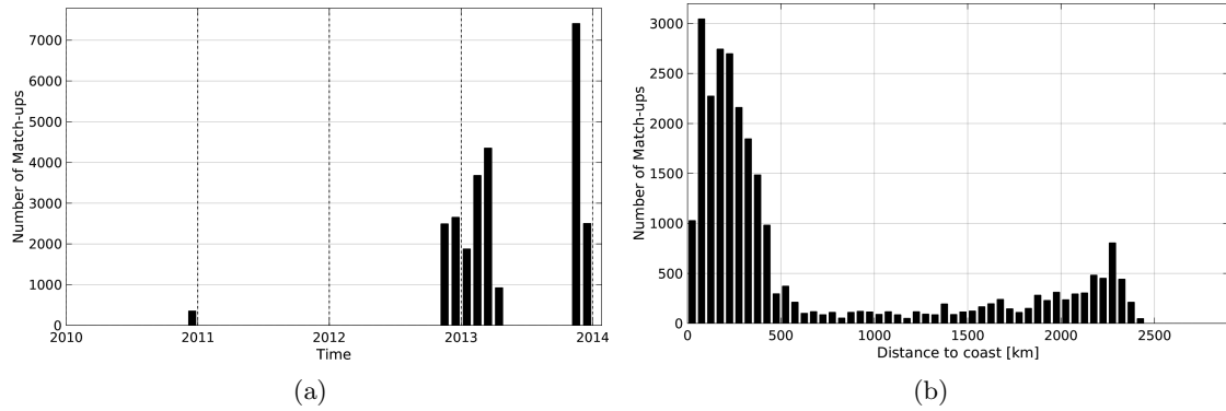
Figure 1: Number of match-ups between TSG-GOSUD-Sailing-ship and SMOS-L3-CATDS-CECOS-IFREMER-V2-1DAY-0.5DEG SSS as a function of time (a) and as function of the distance to coast (b) over the Southern Ocean Pi-MEP region and for the full satellite product period.
