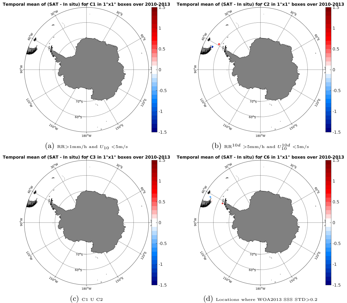
Figure 12: Temporal mean gridded over spatial boxes of size 1^\circ \times 1^\circ of \Delta SSS (SMOS-L3-CATDS-CECOS-IFREMER-V2-1DAY-0.5deg - TSG-GOSUD-Sailing-ship) for 4 different subdatasets corresponding to: RR > 1\text{mm/h} and U_{10} < 5\text{m/s} (a), RR^{10d} > 5\text{mm/h} and U_{10}^{10d} < 5\text{m/s} (b), C1 U C2 (c), Locations where WOA2013 SSS STD > 0.2 (d).
