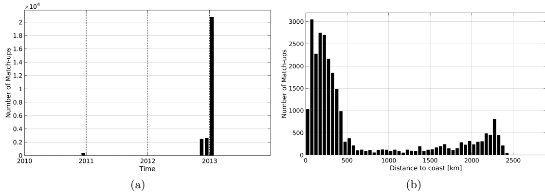
Figure 1: Number of match-ups between TSG-GOSUD-Sailing-ship and SMOS-L3-CATDS-CECOS-IFREMER-V2-1DAY-0.5deg SSS as a function of time (a) and as function of the distance to coast (b) over the Southern Ocean Pi-MEP region and for the full satellite product period.
