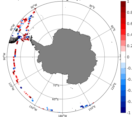
(e) MEAN( \Delta SSS) (Satellite - TSG-GOSUD-Sailing-ship)
