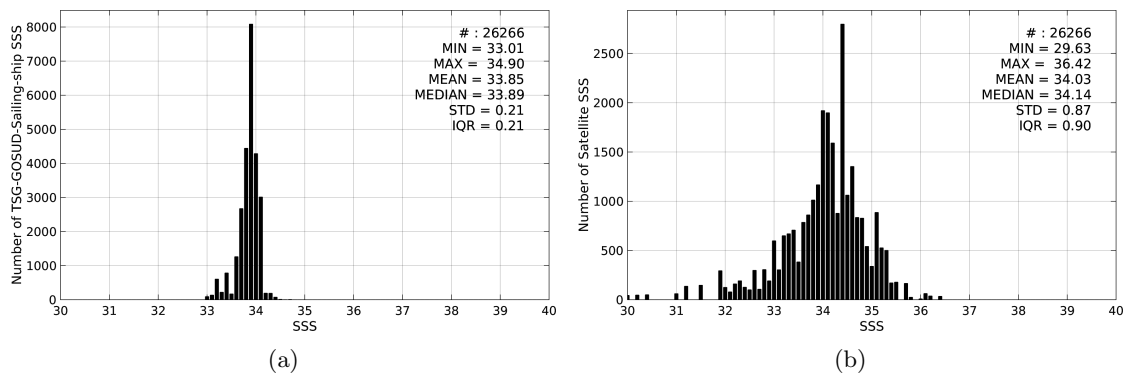
Figure 2: Histograms of SSS from TSG-GOSUD-Sailing-ship (a) and SMOS-L3-CATDS-CECOS-IFREMER-V2-1DAY-0.5deg (b) considering all match-up pairs per bins of 0.1 over the Southern Ocean Pi-MEP region and for the full satellite product period.
