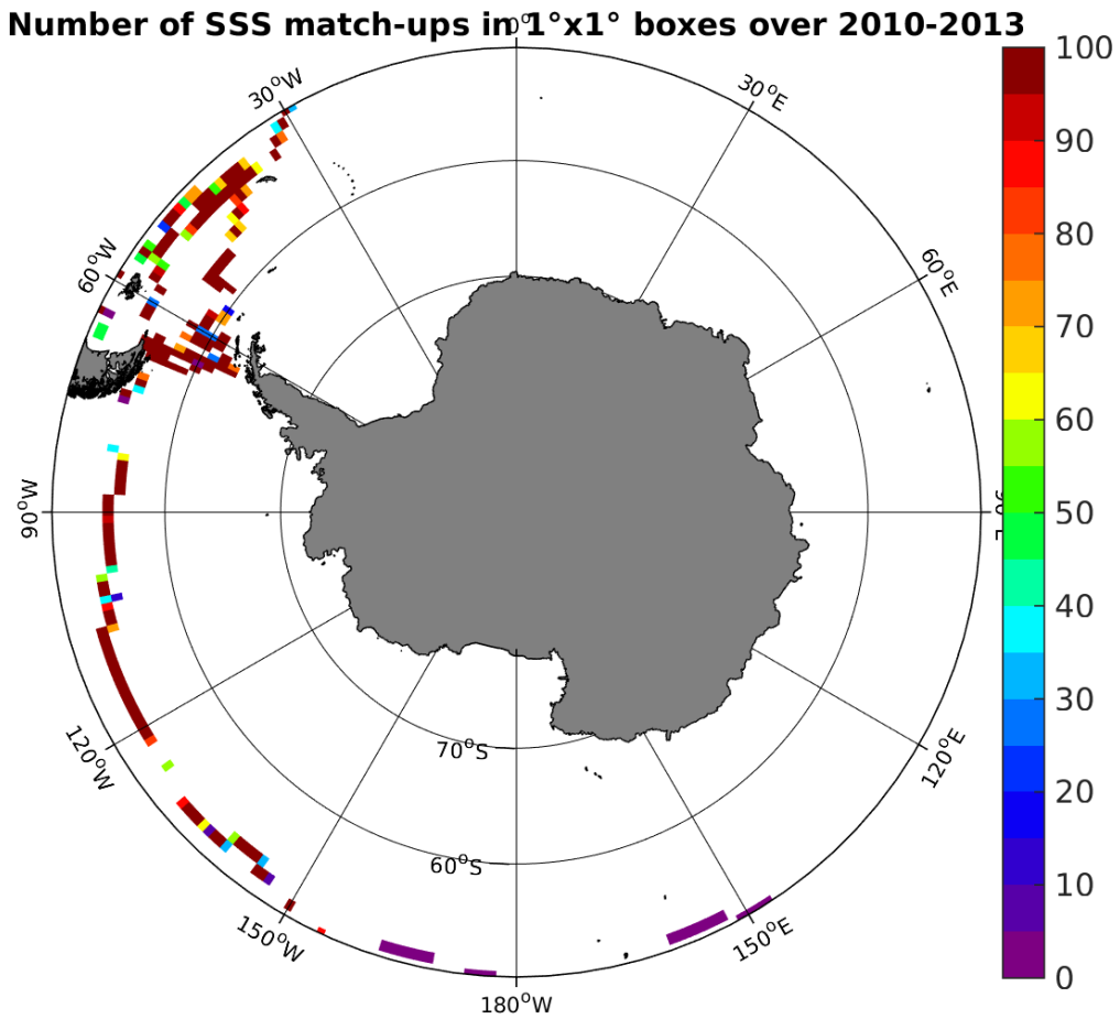
Figure 4: Number of SSS match-ups between TSG-GOSUD-Sailing-ship SSS and the SMOS-L3-CATDS-CECOS-IFREMER-V2-1DAY-0.5deg SSS product for the Southern Ocean Pi-MEP region over 1°x1° boxes and for the full satellite product period.
