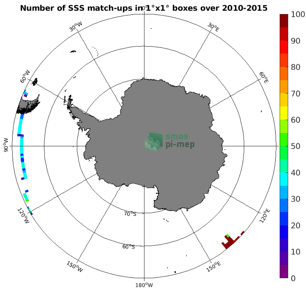
Figure 4: Number of SSS match-ups between TSG (GOSUD-Research-vessel) SSS and the SMOS SSS L3 v2 - Daily - 0.5 Deg (CATDS-CECOS-IFREMER) SSS product for the Southern Ocean Pi-MEP region over 1^\circ \times 1^\circ boxes and for the full satellite product period.
