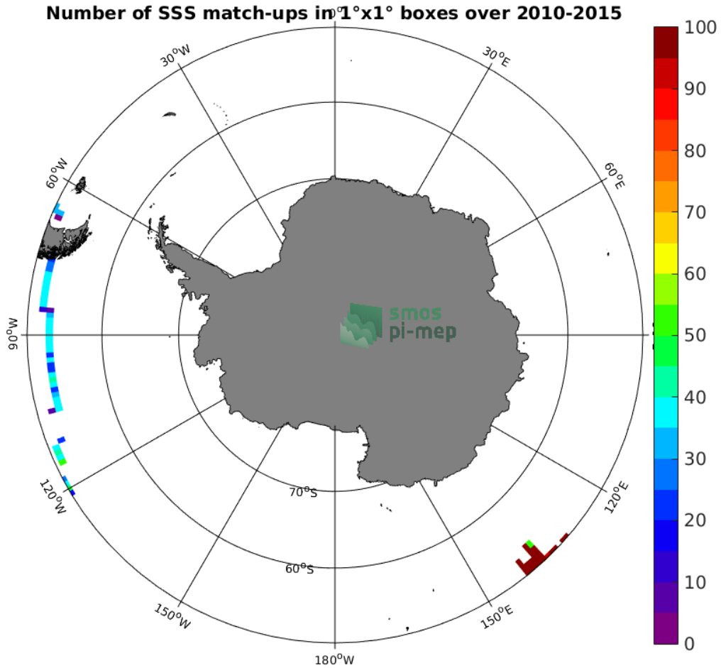
Figure 4: Number of SSS match-ups between TSG (GOSUD-Research-vessel) SSS and the SMOS SSS L3 v2 - Daily - 0.5 Deg (CATDS-CECOS-IFREMER) SSS product for the Southern Ocean Pi-MEP region over 1^\circ \times 1^\circ boxes and for the full satellite product period.
