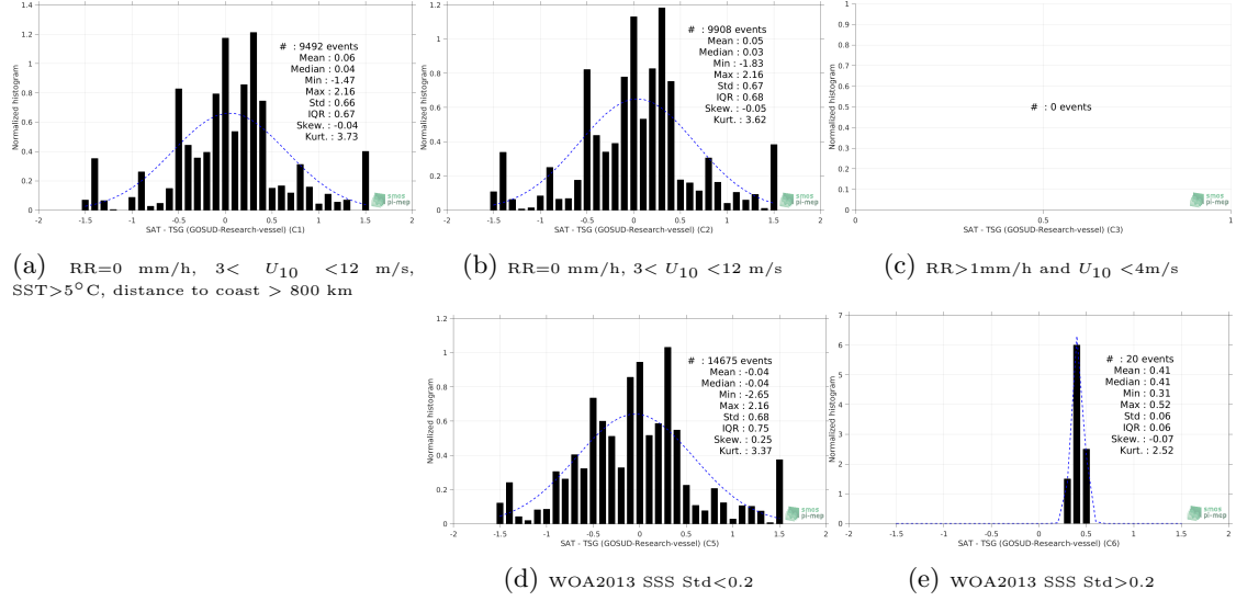
Figure 13: Normalized histogram of \Delta SSS (SMOS SSS L3 v2 - Daily - 0.5 Deg (CATDS-CECOS-IFREMER) - TSG (GOSUD-Research-vessel)) for 5 different subdatasets corresponding to: RR=0 mm/h, 3 < U_{10} < 12 m/s, SST>5°C, distance to coast > 800 km (a), RR=0 mm/h, 3 < U_{10} < 12 m/s (b), RR>1mm/h and U_{10} < 4 m/s (c), WOA2013 SSS Std<0.2 (d), WOA2013 SSS Std>0.2 (e).
