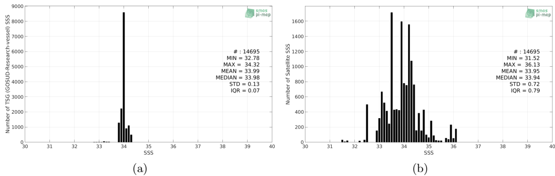
Figure 2: Histograms of SSS from TSG (GOSUD-Research-vessel) (a) and SMOS SSS L3 v2 - Daily - 0.5 Deg (CATDS-CECOS-IFREMER) (b) considering all match-up pairs per bins of 0.1 over the Southern Ocean Pi-MEP region and for the full satellite product period.
