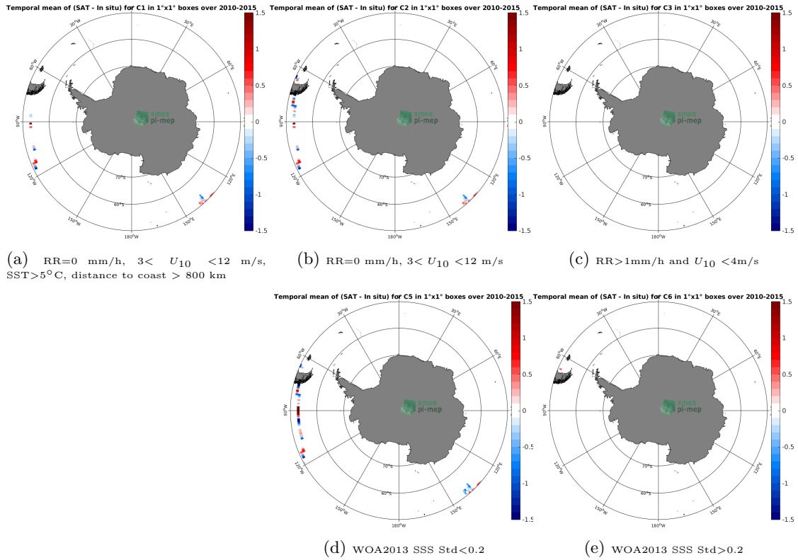
Figure 12: Temporal mean gridded over spatial boxes of size 1°x1° of \Delta SSS (SMOS L3 v2 - Daily - 0.5 Deg (CATDS-CECOS-IFREMER) - TSG-GOSUD-Research-vessel) for 5 different subdatasets corresponding to:RR=0 mm/h, 3 < U_{10} < 12 m/s, SST>5°C, distance to coast > 800 km (a), RR=0 mm/h, 3 < U_{10} < 12 m/s (b), RR>1mm/h and U_{10} < 4 m/s (c), WOA2013 SSS Std<0.2 (d), WOA2013 SSS Std>0.2 (e).
