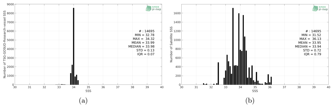
Figure 2: Histograms of SSS from TSG-GOSUD-Research-vessel (a) and SMOS L3 v2 - Daily - 0.5 Deg (CATDS-CECOS-IFREMER) (b) considering all match-up pairs per bins of 0.1 over the Southern Ocean Pi-MEP region and for the full satellite product period.
