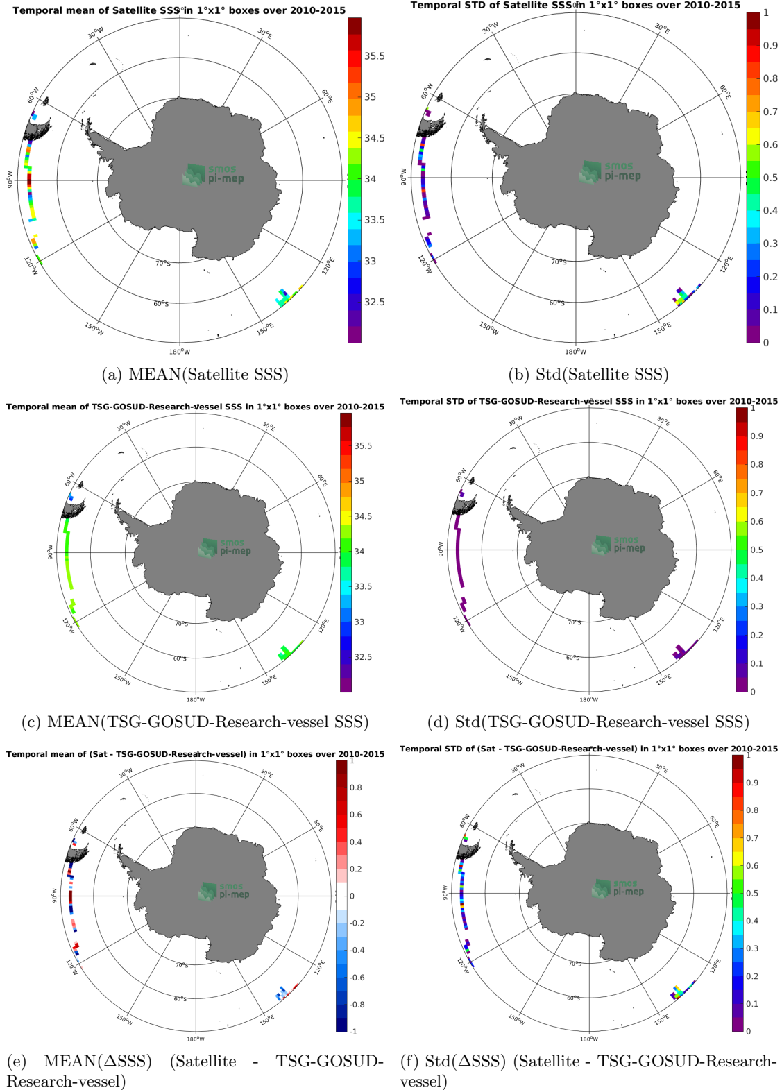
Figure 6: Temporal mean (left) and Std (right) of SSS from SMOS L3 v2 - Daily - 0.5 Deg (CATDS-CECOS-IFREMER) (top), TSG-GOSUD-Research-vessel (middle), and of \Delta SSS (Satellite - TSG-GOSUD-Research-vessel). Only match-up pairs are used to generate these maps.
