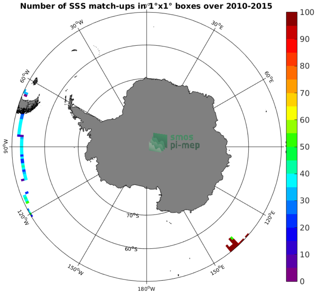
Figure 4: Number of SSS match-ups between TSG-GOSUD-Research-vessel SSS and the SMOS L3 v2 - Daily - 0.5 Deg (CATDS-CECOS-IFREMER) SSS product for the Southern Ocean Pi-MEP region over 1°x1° boxes and for the full satellite product period.
