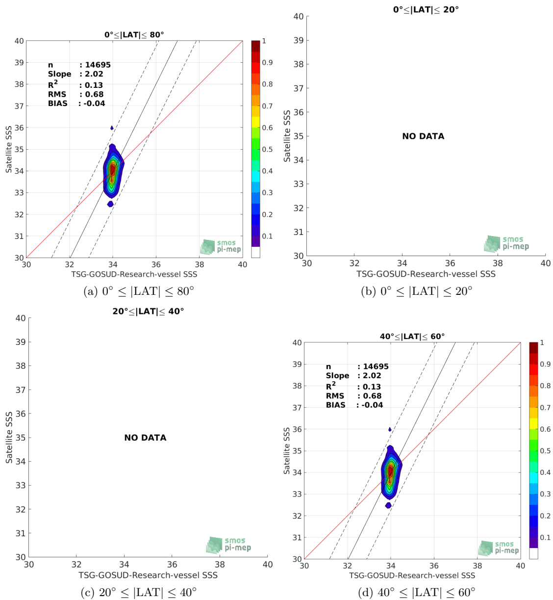
Figure 9: Contour maps of the concentration of SMOS L3 v2 - Daily - 0.5 Deg (CATDS-CECOS-IFREMER) SSS (y-axis) versus TSG-GOSUD-Research-vessel SSS (x-axis) at match-up pairs for different latitude bands. For each plot, the red line shows x=y . The black thin and dashed lines indicate a linear fit through the data cloud and the \pm 95\% confidence levels, respectively. The number match-up pairs n , the slope and R^2 coefficient of the linear fit, the root mean square (RMS) and the mean bias between satellite and in situ data are indicated for each latitude band in each plots.
