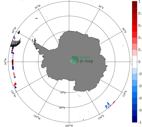
(e) MEAN( \Delta SSS) (Satellite - TSG-GOSUD-Research-vessel)
