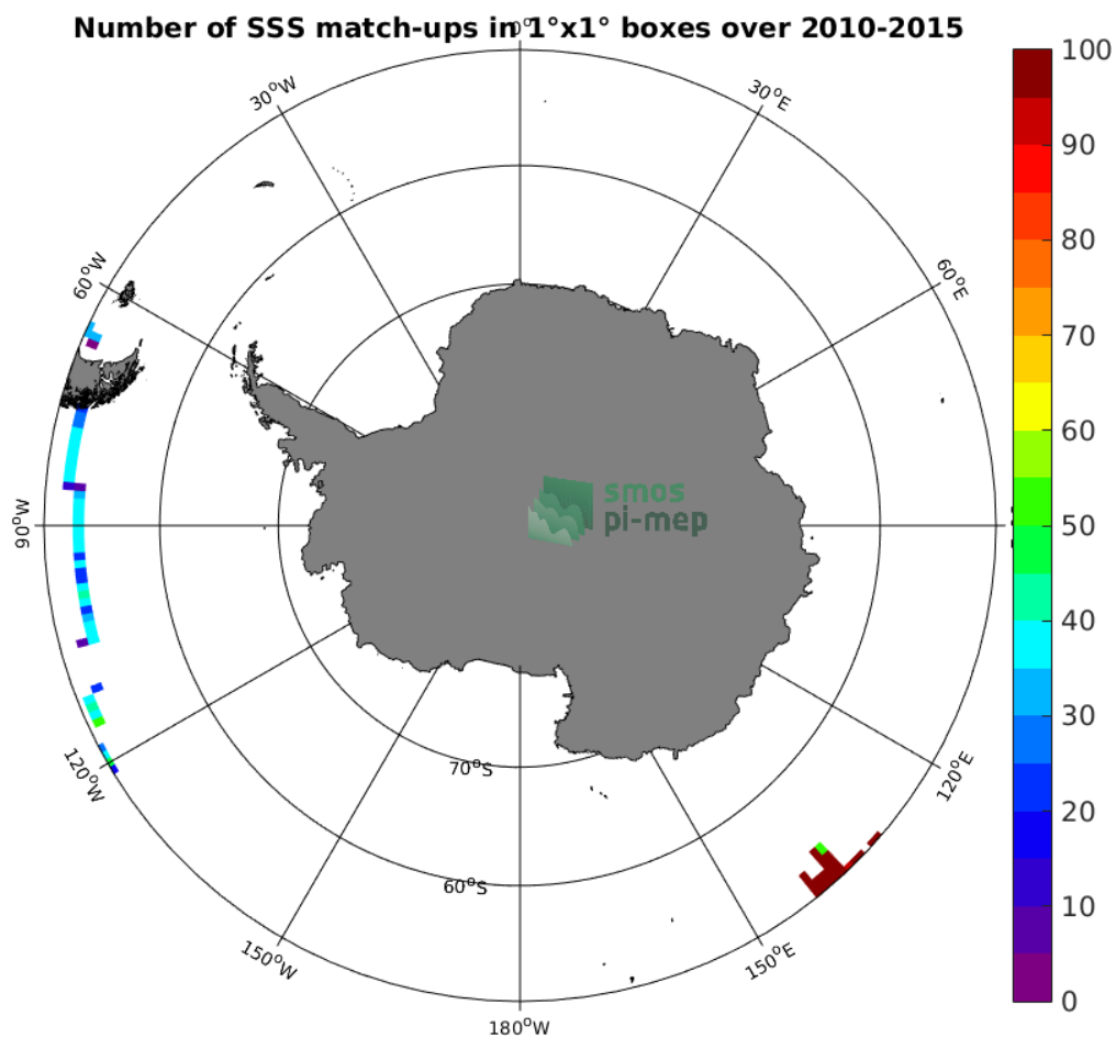
Figure 4: Number of SSS match-ups between TSG-GOSUD-Research-vessel SSS and the SMOS-L3-CATDS-CECOS-IFREMER-V2-1DAY-0.5DEG SSS product for the Southern Ocean Pi-MEP region over 1^\circ \times 1^\circ boxes and for the full satellite product period.
