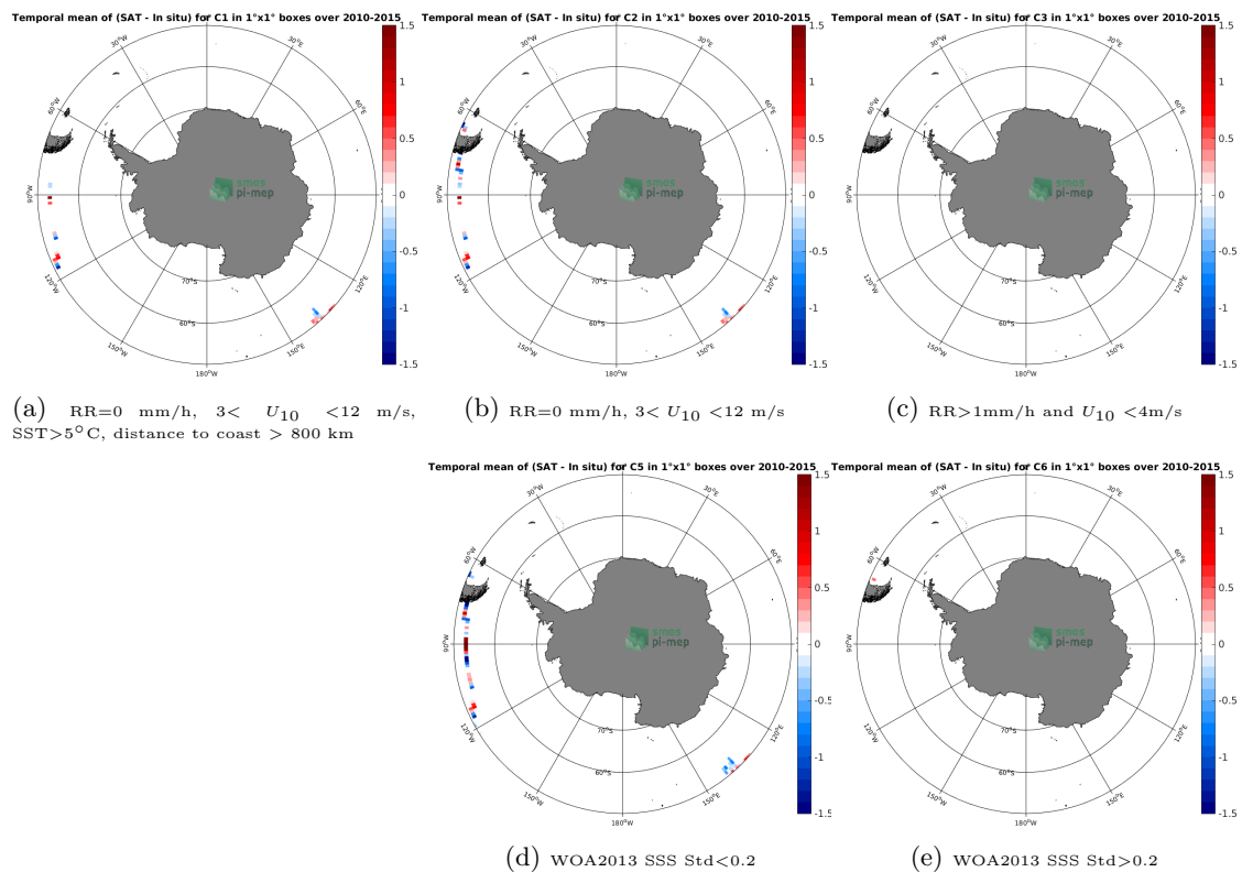
Figure 12: Temporal mean gridded over spatial boxes of size 1^\circ \times 1^\circ of \Delta SSS (SMOS-L3-CATDS-CECOS-IFREMER-V2-1DAY-0.5DEG - TSG-GOSUD-Research-vessel) for 5 different subdatasets corresponding to:RR=0 mm/h, 3 < U_{10} < 12 m/s, SST>5°C, distance to coast > 800 km (a), RR=0 mm/h, 3 < U_{10} < 12 m/s (b), RR>1mm/h and U_{10} < 4 m/s (c), WOA2013 SSS Std<0.2 (d), WOA2013 SSS Std>0.2 (e).
