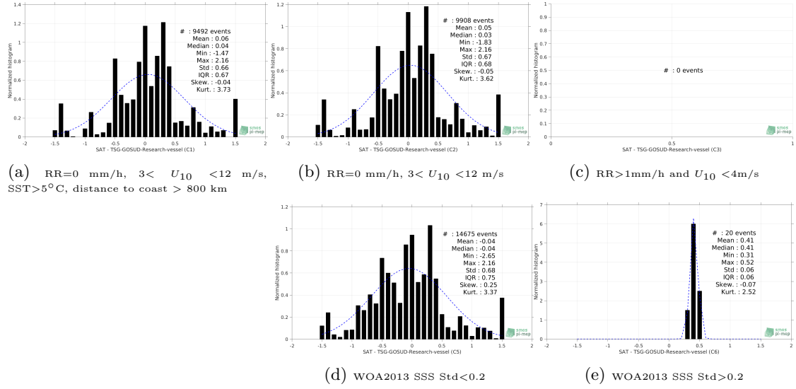
Figure 13: Normalized histogram of \Delta SSS (SMOS-L3-CATDS-CECOS-IFREMER-V2-1DAY-0.5DEG - TSG-GOSUD-Research-vessel) for 5 different subdatasets corresponding to: RR=0 mm/h, 3 < U_{10} < 12 m/s, SST > 5°C, distance to coast > 800 km (a), RR=0 mm/h, 3 < U_{10} < 12 m/s (b), RR > 1mm/h and U_{10} < 4 m/s (c), WOA2013 SSS Std < 0.2 (d), WOA2013 SSS Std > 0.2 (e).
