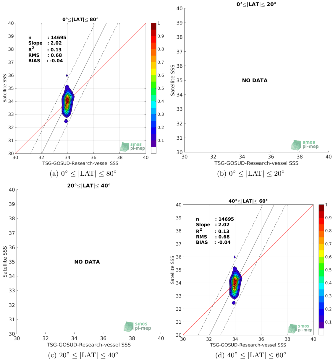
Figure 9: Contour maps of the concentration of SMOS-L3-CATDS-CECOS-IFREMER-V2-1DAY-0.5DEG SSS (y-axis) versus TSG-GOSUD-Research-vessel SSS (x-axis) at match-up pairs for different latitude bands. For each plot, the red line shows x=y . The black thin and dashed lines indicate a linear fit through the data cloud and the \pm 95\% confidence levels, respectively. The number match-up pairs n , the slope and R^2 coefficient of the linear fit, the root mean square (RMS) and the mean bias between satellite and in situ data are indicated for each latitude band in each plots.
