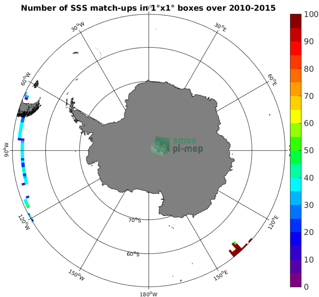
Figure 4: Number of SSS match-ups between TSG-GOSUD-Research-vessel SSS and the SMOS-L3-CATDS-CECOS-IFREMER-V2-1DAY-0.5DEG SSS product for the Southern Ocean Pi-MEP region over 1°x1° boxes and for the full satellite product period.
