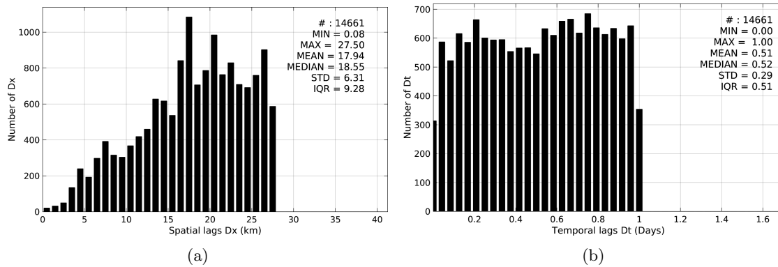
Figure 5: Histograms of the spatial (a) and temporal (b) lags between the time of the TSG-GOSUD-Research-vessel measurements and the date of the corresponding SMOS-L3-CATDS-CECOS-IFREMER-V2-1DAY-0.5deg SSS product.
