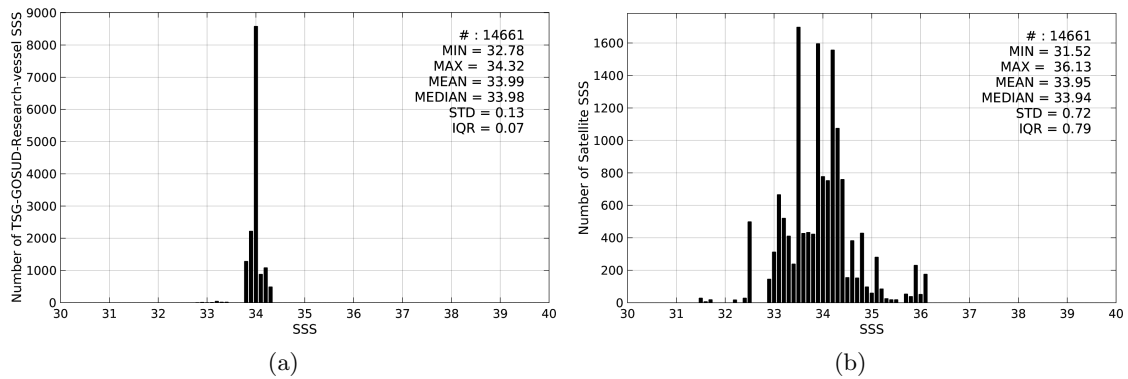
Figure 2: Histograms of SSS from TSG-GOSUD-Research-vessel (a) and SMOS-L3-CATDS-CECOS-IFREMER-V2-1DAY-0.5deg (b) considering all match-up pairs per bins of 0.1 over the Southern Ocean Pi-MEP region and for the full satellite product period.
