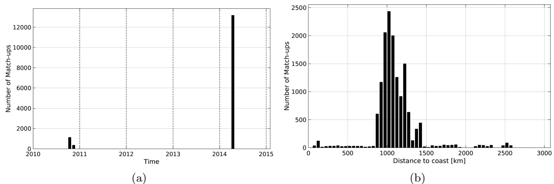
Figure 1: Number of match-ups between TSG-GOSUD-Research-vessel and SMOS-L3-CATDS-CECOS-IFREMER-V2-1DAY-0.5deg SSS as a function of time (a) and as function of the distance to coast (b) over the Southern Ocean Pi-MEP region and for the full satellite product period.
