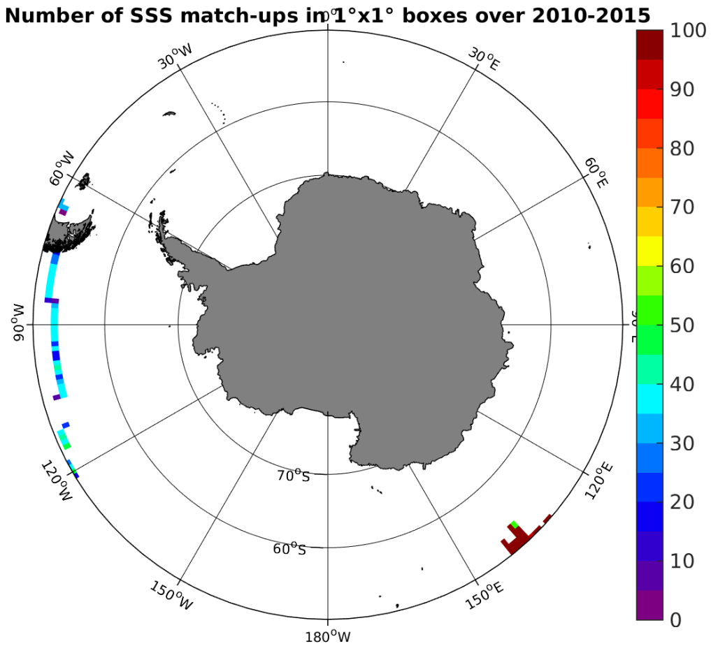
Figure 4: Number of SSS match-ups between TSG-GOSUD-Research-vessel SSS and the SMOS-L3-CATDS-CECOS-IFREMER-V2-1DAY-0.5deg SSS product for the Southern Ocean Pi-MEP region over 1°x1° boxes and for the full satellite product period.
