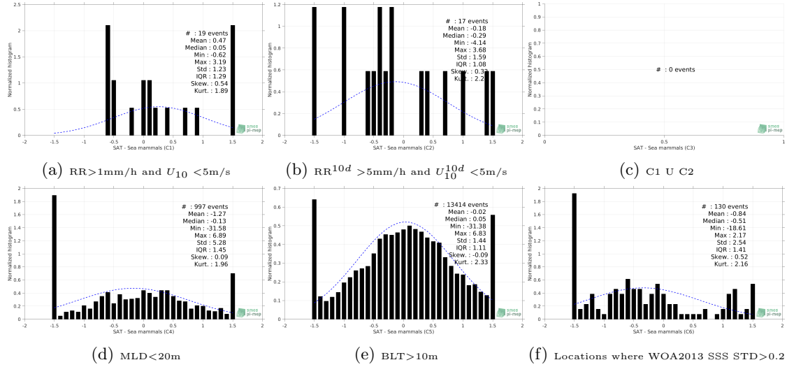
Figure 13: Normalized histogram of \Delta SSS (SMOS-L3-CATDS-CECOS-IFREMER-V2-1DAY-0.5DEG - Sea mammals) for 6 different subdatasets corresponding to: RR>1mm/h and U_{10} < 5\text{m/s} (a), RR^{10d} > 5\text{mm/h} and U_{10}^{10d} < 5\text{m/s} (b), C1 U C2 (c),MLD<20m (d),BLT>10m (e),Locations where WOA2013 SSS STD>0.2 (f).
