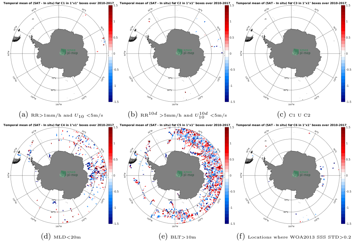
Figure 12: Temporal mean gridded over spatial boxes of size 1^\circ \times 1^\circ of \Delta\text{SSS} (SMOS-L3-CATDS-CECOS-IFREMER-V2-1DAY-0.5DEG - Sea mammals) for 6 different subdatasets corresponding to: \text{RR} > 1\text{mm/h} and U_{10} < 5\text{m/s} (a), \text{RR}^{10d} > 5\text{mm/h} and U_{10}^{10d} < 5\text{m/s} (b), C1 U C2 (c), \text{MLD} < 20\text{m} (d), \text{BLT} > 10\text{m} (e), Locations where WOA2013 SSS STD > 0.2 (f).
