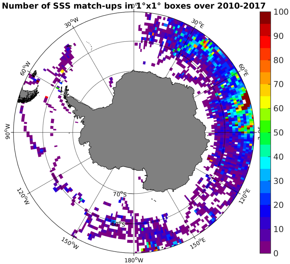
Figure 4: Number of SSS match-ups between Sea mammals SSS and the SMOS-L3-CATDS-CECOS-IFREMER-V2-1DAY-0.5DEG SSS product for the Southern Ocean Pi-MEP region over 1°x1° boxes and for the full satellite product period.
