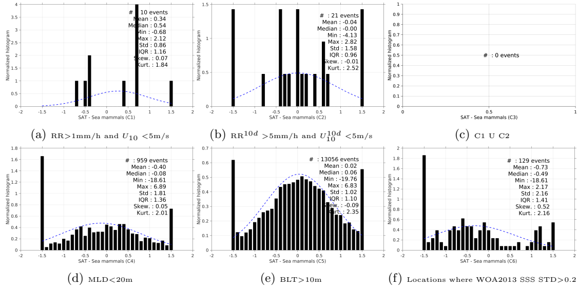
Figure 13: Normalized histogram of \Delta SSS (SMOS-L3-CATDS-CECOS-IFREMER-V2-1DAY-0.5DEG - Sea mammals) for 6 different subdatasets corresponding to: RR>1mm/h and U_{10} < 5\text{m/s} (a), RR^{10d} > 5\text{mm/h} and U_{10}^{10d} < 5\text{m/s} (b), C1 U C2 (c),MLD<20m (d),BLT>10m (e),Locations where WOA2013 SSS STD>0.2 (f).
