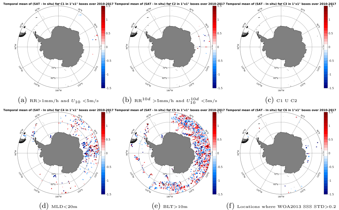
Figure 12: Temporal mean gridded over spatial boxes of size 1^\circ \times 1^\circ of \Delta SSS (SMOS-L3-CATDS-CECOS-IFREMER-V2-1DAY-0.5DEG - Sea mammals) for 6 different subdatasets corresponding to: RR > 1\text{mm/h} and U_{10} < 5\text{m/s} (a), RR^{10d} > 5\text{mm/h} and U_{10}^{10d} < 5\text{m/s} (b), C1 U C2 (c), MLD < 20\text{m} (d), BLT > 10\text{m} (e), Locations where WOA2013 SSS STD > 0.2 (f).
