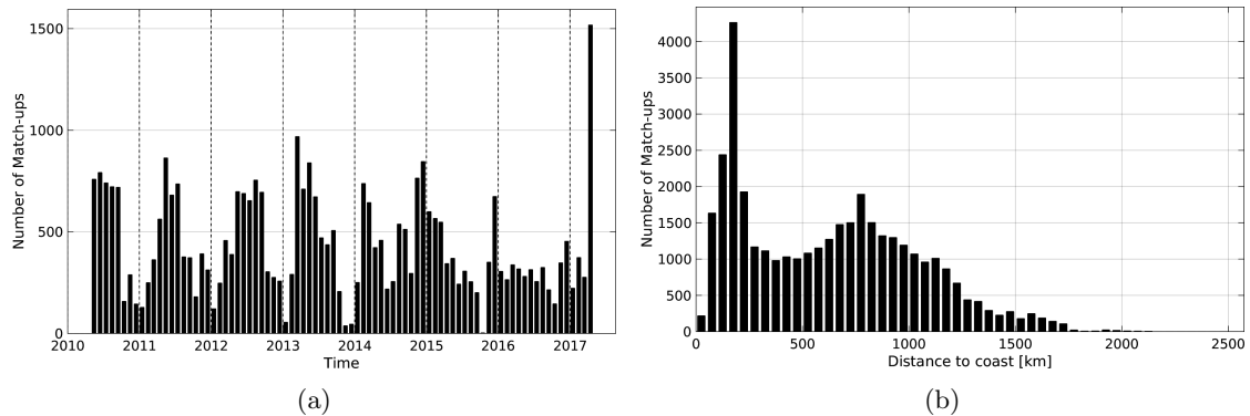
Figure 1: Number of match-ups between Sea mammals and SMOS-L3-CATDS-CECOS-IFREMER-V2-1DAY-0.5deg SSS as a function of time (a) and as function of the distance to coast (b) over the Southern Ocean Pi-MEP region and for the full satellite product period.
