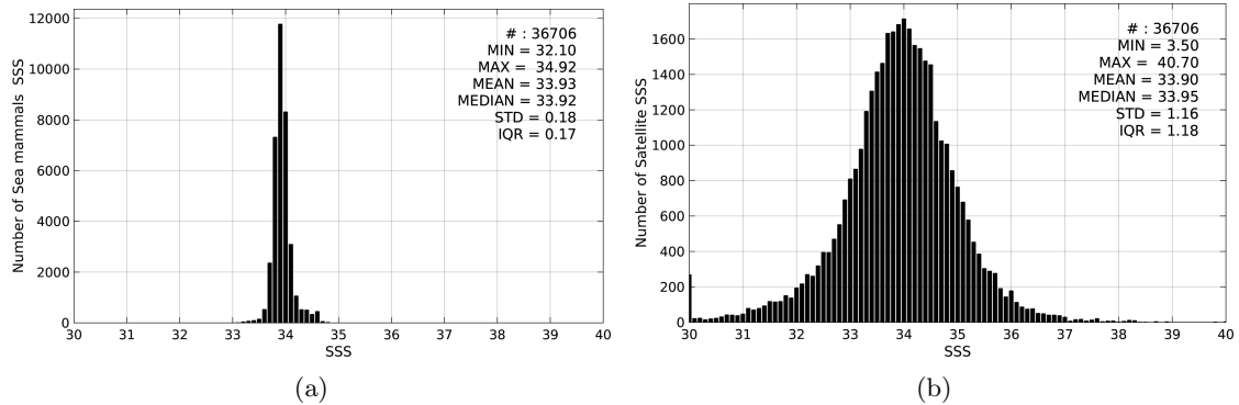
Figure 2: Histograms of SSS from Sea mammals (a) and SMOS-L3-CATDS-CECOS-IFREMER-V2-1DAY-0.5deg (b) considering all match-up pairs per bins of 0.1 over the Southern Ocean Pi-MEP region and for the full satellite product period.
