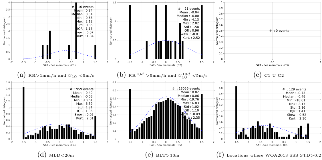
Figure 13: Normalized histogram of \Delta SSS (SMOS-L3-CATDS-CECOS-IFREMER-V2-1DAY-0.5deg - Sea mammals) for 6 different subdatasets corresponding to: RR > 1\text{mm/h} and U_{10} < 5\text{m/s} (a), RR^{10d} > 5\text{mm/h} and U_{10}^{10d} < 5\text{m/s} (b), C1 \cup C2 (c), MLD < 20\text{m} (d), BLT > 10\text{m} (e), Locations where WOA2013 SSS STD > 0.2 (f).
