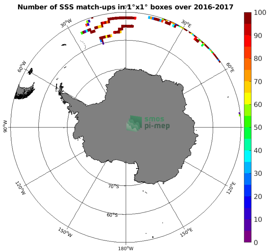
Figure 3: Number of SSS match-ups between Surface drifters SSS and the SMOS SSS L3 v2 - Daily - 0.5 Deg (CATDS-CECOS-IFREMER) SSS product for the Southern Ocean Pi-MEP region over 1^\circ \times 1^\circ boxes and for the full satellite product period.
