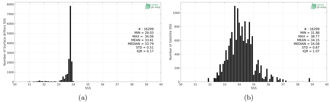
Figure 2: Histograms of SSS from Surface drifters (a) and SMOS SSS L3 v2 - Daily - 0.5 Deg (CATDS-CECOS-IFREMER) (b) considering all match-up pairs per bins of 0.1 over the Southern Ocean Pi-MEP region and for the full satellite product period.
