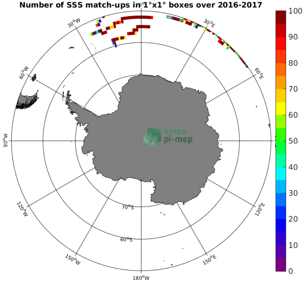
Figure 3: Number of SSS match-ups between Surface drifters SSS and the SMOS SSS L3 v2 - Daily - 0.5 Deg (CATDS-CECOS-IFREMER) SSS product for the Southern Ocean Pi-MEP region over 1°x1° boxes and for the full satellite product period.
