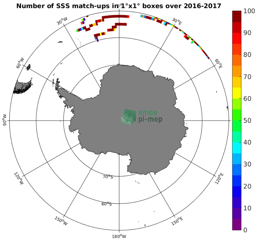
Figure 3: Number of SSS match-ups between Surface drifters SSS and the SMOS L3 v2 - Daily - 0.5 Deg (CATDS-CECOS-IFREMER) SSS product for the Southern Ocean Pi-MEP region over 1^\circ \times 1^\circ boxes and for the full satellite product period.
