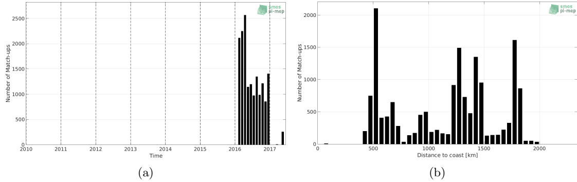
Figure 1: Number of match-ups between Surface drifters and SMOS L3 v2 - Daily - 0.5 Deg (CATDS-CECOS-IFREMER) SSS as a function of time (a) and as function of the distance to coast (b) over the Southern Ocean Pi-MEP region and for the full satellite product period.
