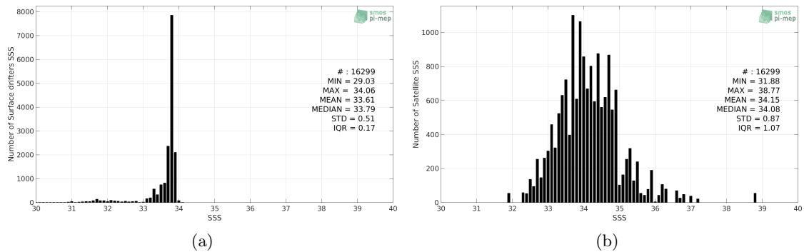
Figure 2: Histograms of SSS from Surface drifters (a) and SMOS L3 v2 - Daily - 0.5 Deg (CATDS-CECOS-IFREMER) (b) considering all match-up pairs per bins of 0.1 over the Southern Ocean Pi-MEP region and for the full satellite product period.
