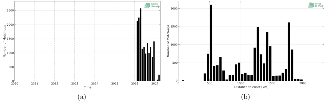
Figure 1: Number of match-ups between Surface drifters and SMOS-L3-CATDS-CECOS-IFREMER-V2-1DAY-0.5DEG SSS as a function of time (a) and as function of the distance to coast (b) over the Southern Ocean Pi-MEP region and for the full satellite product period.
