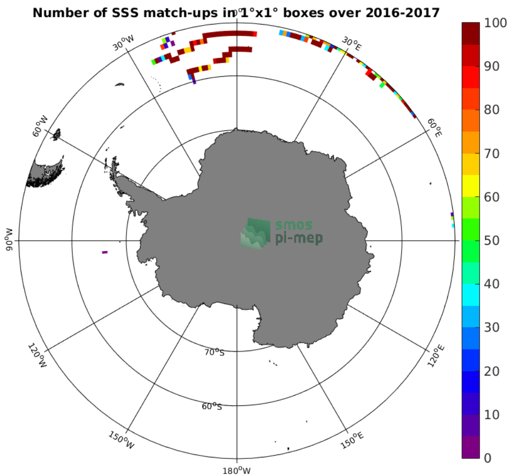
Figure 3: Number of SSS match-ups between Surface drifters SSS and the SMOS-L3-CATDS-CECOS-IFREMER-V2-1DAY-0.5DEG SSS product for the Southern Ocean Pi-MEP region over 1°x1° boxes and for the full satellite product period.
