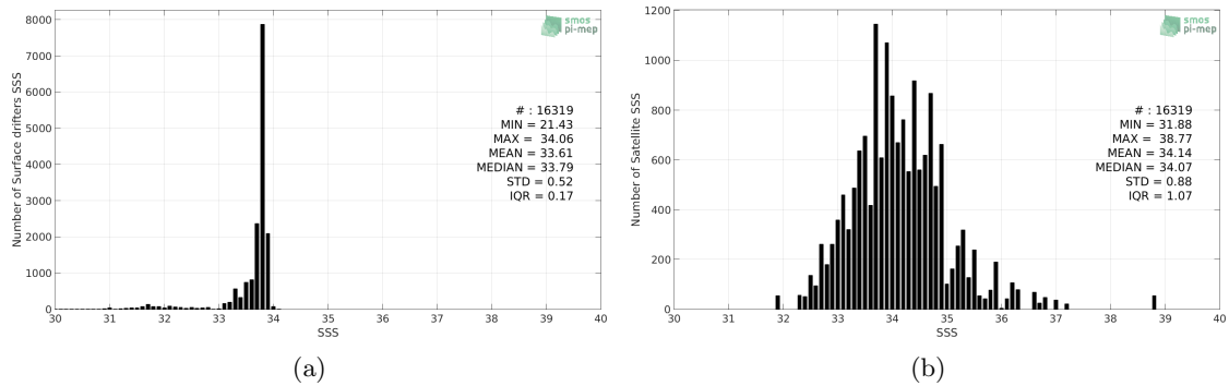
Figure 2: Histograms of SSS from Surface drifters (a) and SMOS-L3-CATDS-CECOS-IFREMER-V2-1DAY-0.5DEG (b) considering all match-up pairs per bins of 0.1 over the Southern Ocean Pi-MEP region and for the full satellite product period.
