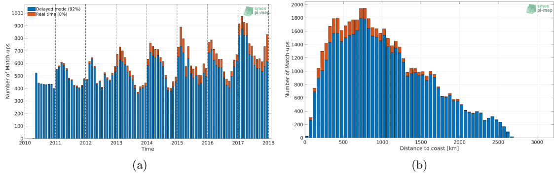
Figure 1: Number of match-ups between Argo and SMOS SSS L3 v2 - Daily - 0.5 Deg (CATDS-CECOS-IFREMER) SSS as a function of time (a) and as function of the distance to coast (b) over the Southern Ocean Pi-MEP region and for the full satellite product period.
