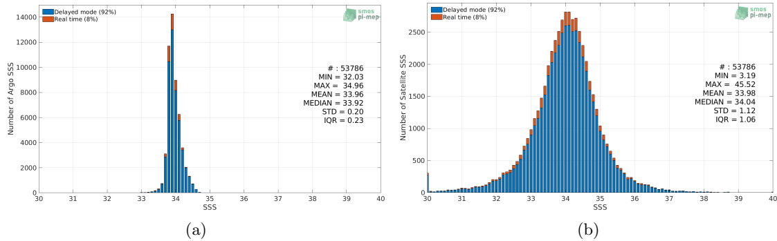
Figure 2: Histograms of SSS from Argo (a) and SMOS SSS L3 v2 - Daily - 0.5 Deg (CATDS-CECOS-IFREMER) (b) considering all match-up pairs per bins of 0.1 over the Southern Ocean Pi-MEP region and for the full satellite product period.
