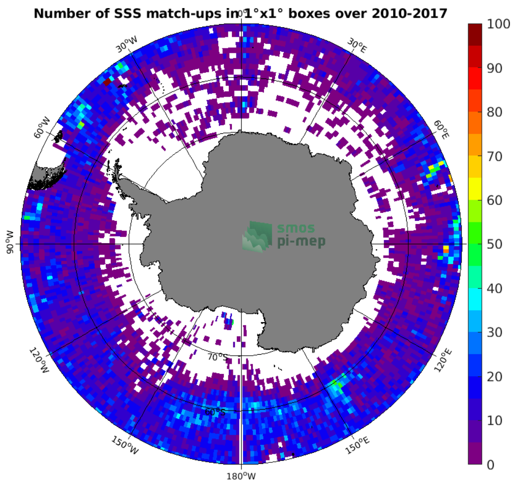
Figure 4: Number of SSS match-ups between Argo SSS and the SMOS SSS L3 v2 - Daily - 0.5 Deg (CATDS-CECOS-IFREMER) SSS product for the Southern Ocean Pi-MEP region over 1^{\circ} \times 1^{\circ} boxes and for the full satellite product period.
