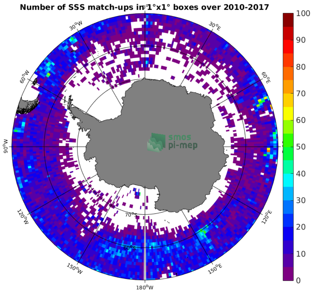
Figure 4: Number of SSS match-ups between Argo SSS and the SMOS SSS L3 v2 - Daily - 0.5 Deg (CATDS-CECOS-IFREMER) SSS product for the Southern Ocean Pi-MEP region over 1^\circ \times 1^\circ boxes and for the full satellite product period.
