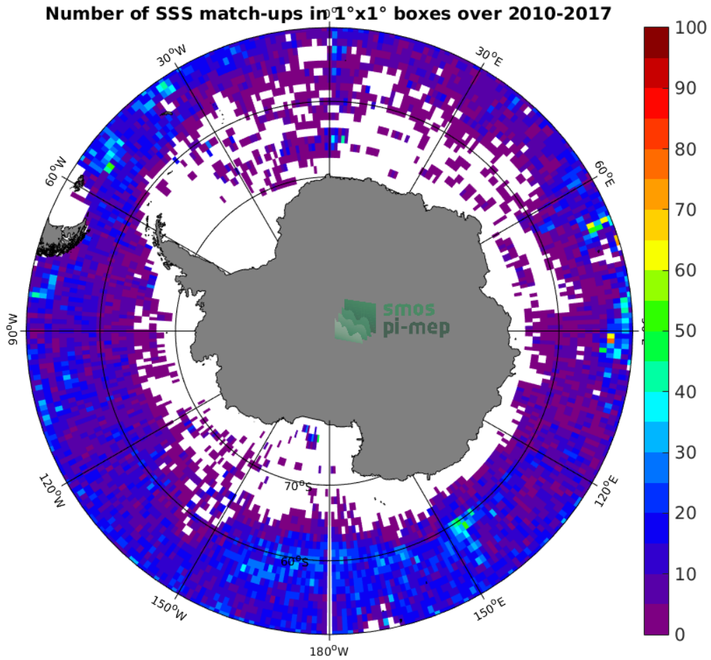
Figure 4: Number of SSS match-ups between Argo SSS and the SMOS-L3-CATDS-CECOS-IFREMER-V2-1DAY-0.5DEG SSS product for the Southern Ocean Pi-MEP region over 1°x1° boxes and for the full satellite product period.
