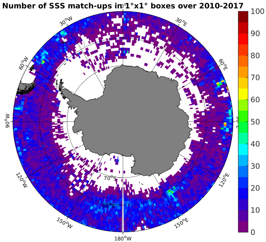
Figure 4: Number of SSS match-ups between Argo SSS and the SMOS-L3-CATDS-CECOS-IFREMER-V2-1DAY-0.5deg SSS product for the Southern Ocean Pi-MEP region over 1^\circ \times 1^\circ boxes and for the full satellite product period.
