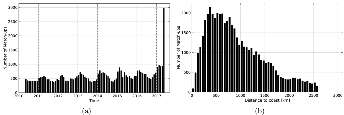
Figure 1: Number of match-ups between Argo and SMOS-L3-CATDS-CECOS-IFREMER-V2-1DAY-0.5deg SSS as a function of time (a) and as function of the distance to coast (b) over the Southern Ocean Pi-MEP region and for the full satellite product period.
