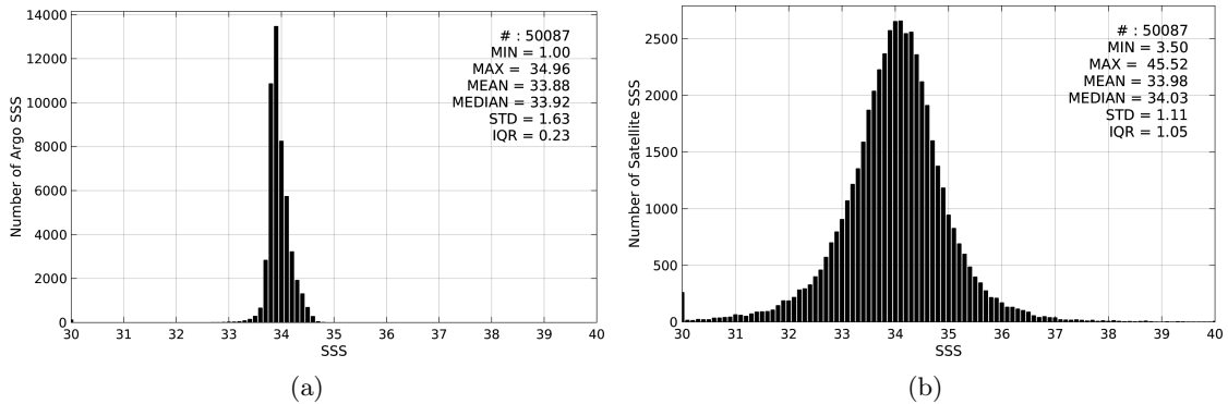
Figure 2: Histograms of SSS from Argo (a) and SMOS-L3-CATDS-CECOS-IFREMER-V2-1DAY-0.5deg (b) considering all match-up pairs per bins of 0.1 over the Southern Ocean Pi-MEP region and for the full satellite product period.
