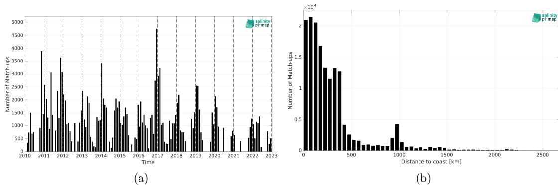
Figure 2: Number of match-ups between TSG (SAMOS) and SMOS SSS L3 v335 - Monthly - 25 km (CATDS-CPDC) SSS as a function of time (a) and as function of the distance to coast (b) over the Southern Ocean Pi-MEP region and for the full satellite product period.
