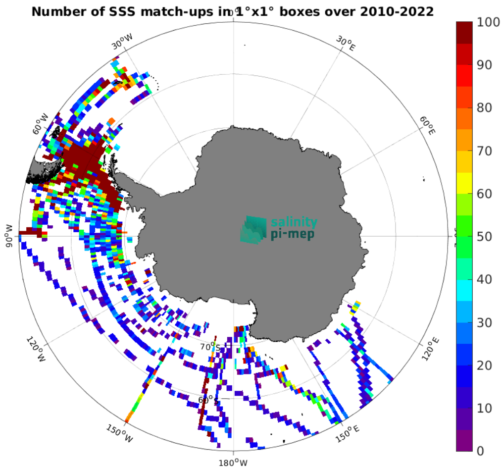
Figure 5: Number of SSS match-ups between TSG (SAMOS) SSS and the SMOS SSS L3 v335 - Monthly - 25 km (CATDS-CPDC) SSS product for the Southern Ocean Pi-MEP region over 1^{\circ} \times 1^{\circ} boxes and for the full satellite product period.
