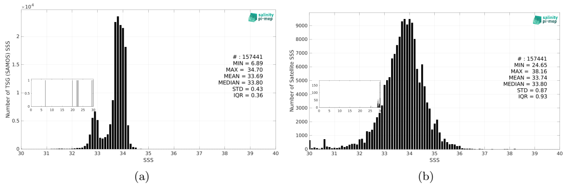
Figure 3: Histograms of SSS from TSG (SAMOS) (a) and SMOS SSS L3 v335 - Monthly - 25 km (CATDS-CPDC) (b) considering all match-up pairs per bins of 0.1 over the Southern Ocean Pi-MEP region and for the full satellite product period.
