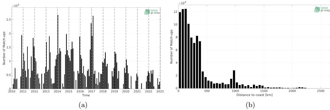
Figure 1: Number of match-ups between TSG (SAMOS) and SMOS SSS L3 v335 - Monthly - 25 km (CATDS-CPDC) SSS as a function of time (a) and as function of the distance to coast (b) over the Southern Ocean Pi-MEP region and for the full satellite product period.
