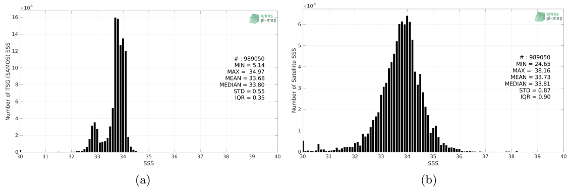
Figure 2: Histograms of SSS from TSG (SAMOS) (a) and SMOS SSS L3 v335 - Monthly - 25 km (CATDS-CPDC) (b) considering all match-up pairs per bins of 0.1 over the Southern Ocean Pi-MEP region and for the full satellite product period.
