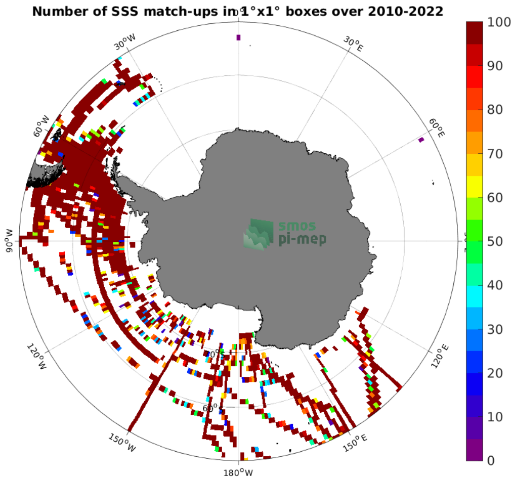
Figure 4: Number of SSS match-ups between TSG (SAMOS) SSS and the SMOS SSS L3 v335 - Monthly - 25 km (CATDS-CPDC) SSS product for the Southern Ocean Pi-MEP region over 1^\circ \times 1^\circ boxes and for the full satellite product period.
