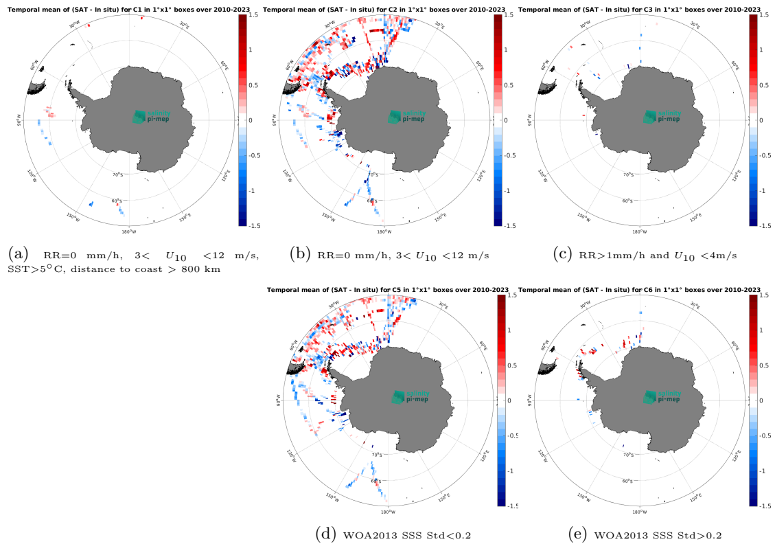
Figure 14: Temporal mean gridded over spatial boxes of size 1^\circ \times 1^\circ of \Delta SSS (SMOS SSS L3 v335 - Monthly - 25 km (CATDS-CPDC) - TSG (Polarstern)) for 5 different subdatasets corresponding to:RR=0 mm/h, 3 < U_{10} < 12 m/s, SST >5^\circ C, distance to coast > 800 km (a), RR=0 mm/h, 3 < U_{10} < 12 m/s (b), RR >1 mm/h and U_{10} < 4 m/s (c), WOA2013 SSS Std <0.2 (d), WOA2013 SSS Std >0.2 (e).
