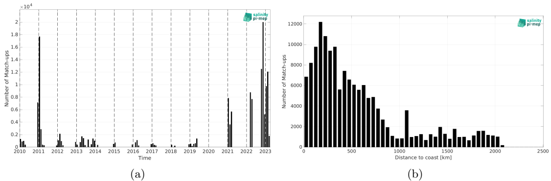
Figure 2: Number of match-ups between TSG (Polarstern) and SMOS SSS L3 v335 - Monthly - 25 km (CATDS-CPDC) SSS as a function of time (a) and as function of the distance to coast (b) over the Southern Ocean Pi-MEP region and for the full satellite product period.
