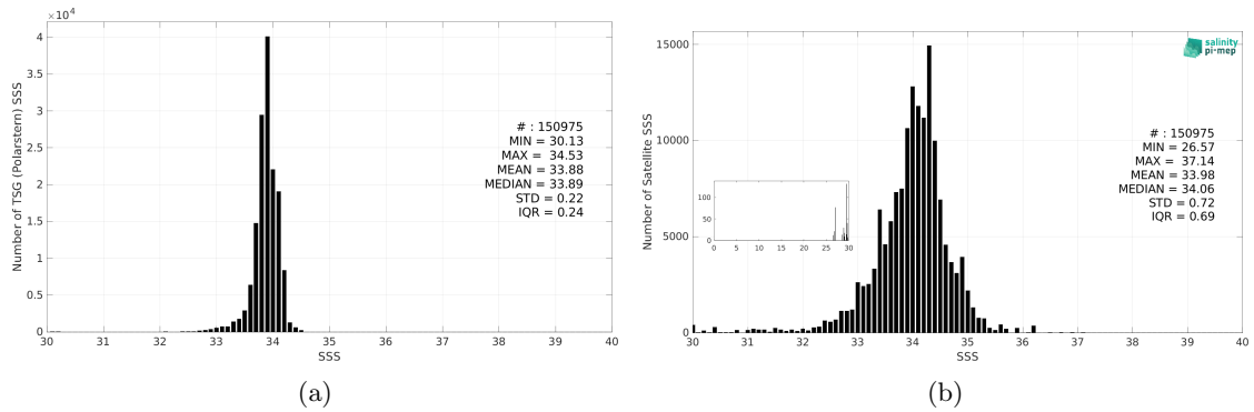
Figure 3: Histograms of SSS from TSG (Polarstern) (a) and SMOS SSS L3 v335 - Monthly - 25 km (CATDS-CPDC) (b) considering all match-up pairs per bins of 0.1 over the Southern Ocean Pi-MEP region and for the full satellite product period.
