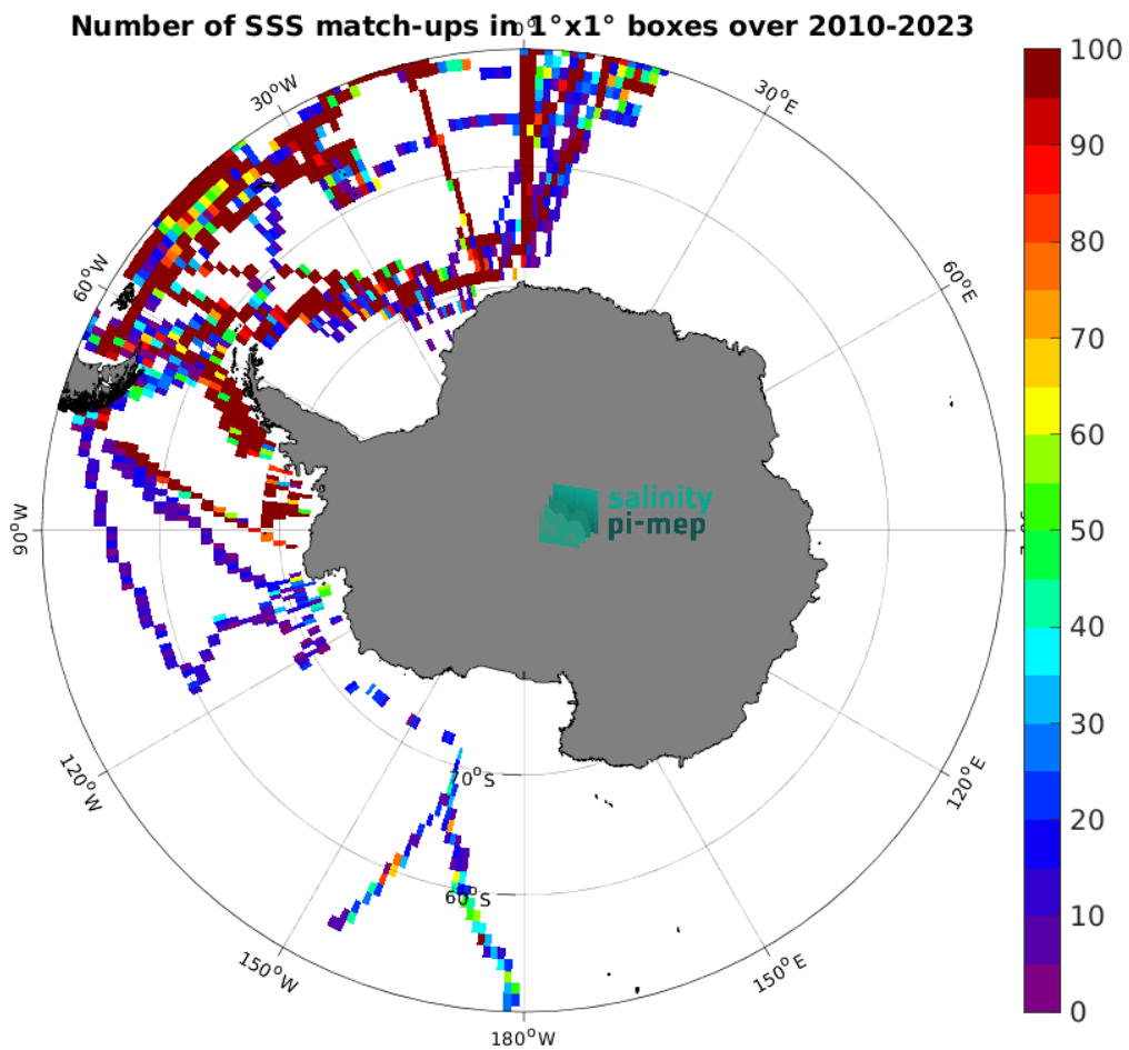
Figure 5: Number of SSS match-ups between TSG (Polarstern) SSS and the SMOS SSS L3 v335 - Monthly - 25 km (CATDS-CPDC) SSS product for the Southern Ocean Pi-MEP region over 1^\circ \times 1^\circ boxes and for the full satellite product period.
