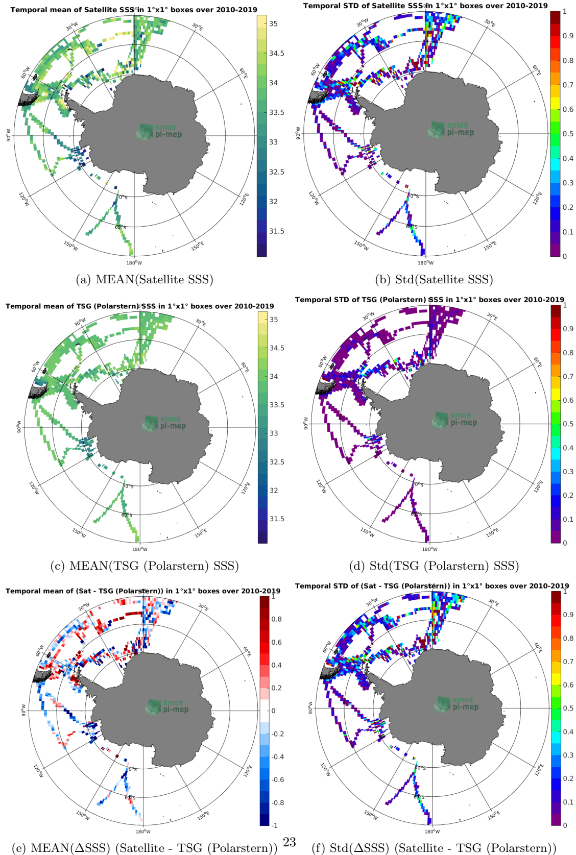
Figure 6: Temporal mean (left) and Std (right) of SSS from SMOS SSS L3 v335 - Monthly - 25 km (CATDS-CPDC) (top), TSG (Polarstern) (middle), and of \Delta SSS (Satellite - TSG (Polarstern)). Only match-up pairs are used to generate these maps.
