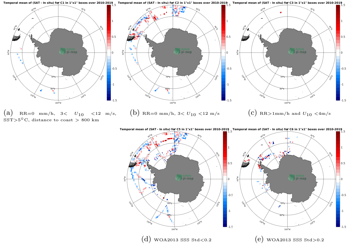
Figure 12: Temporal mean gridded over spatial boxes of size 1^{\circ} \times 1^{\circ} of \Delta\text{SSS} (SMOS SSS L3 v335 - Monthly - 25 km (CATDS-CPDC) - TSG (Polarstern)) for 5 different subdatasets corresponding to: RR=0 mm/h, 3 < U_{10} < 12 m/s, SST >5^{\circ}\text{C} , distance to coast > 800 km (a), RR=0 mm/h, 3 < U_{10} < 12 m/s (b), RR >1 mm/h and U_{10} < 4 m/s (c), WOA2013 SSS Std <0.2 (d), WOA2013 SSS Std >0.2 (e).
