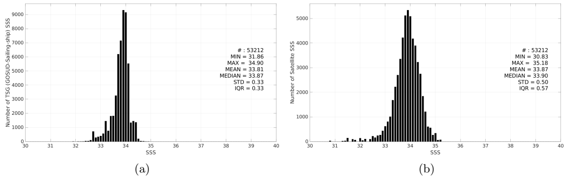
Figure 3: Histograms of SSS from TSG (GOSUD-Sailing-ship) (a) and SMOS SSS L3 v335 - Monthly - 25 km (CATDS-CPDC) (b) considering all match-up pairs per bins of 0.1 over the Southern Ocean Pi-MEP region and for the full satellite product period.
