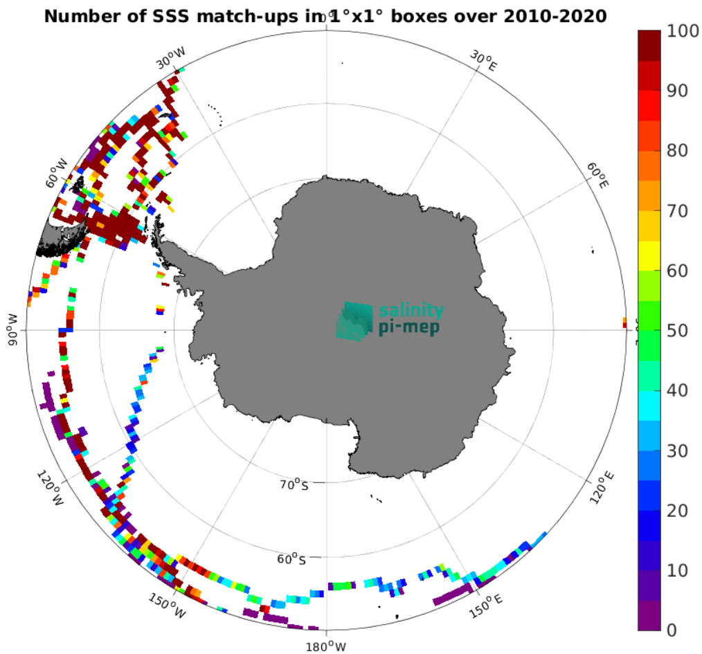
Figure 5: Number of SSS match-ups between TSG (GOSUD-Sailing-ship) SSS and the SMOS SSS L3 v335 - Monthly - 25 km (CATDS-CPDC) SSS product for the Southern Ocean Pi-MEP region over 1^{\circ} \times 1^{\circ} boxes and for the full satellite product period.
