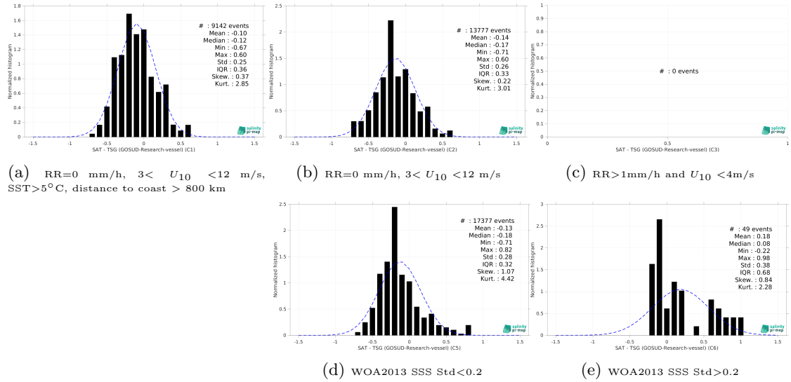
Figure 15: Normalized histogram of \Delta SSS (SMOS SSS L3 v335 - Monthly - 25 km (CATDS-CPDC) - TSG (GOSUD-Research-vessel)) for 5 different subdatasets corresponding to: RR=0 mm/h, 3 < U_{10} < 12 m/s, SST > 5°C, distance to coast > 800 km (a), RR=0 mm/h, 3 < U_{10} < 12 m/s (b), RR > 1mm/h and U_{10} < 4 m/s (c), WOA2013 SSS Std < 0.2 (d), WOA2013 SSS Std > 0.2 (e).
