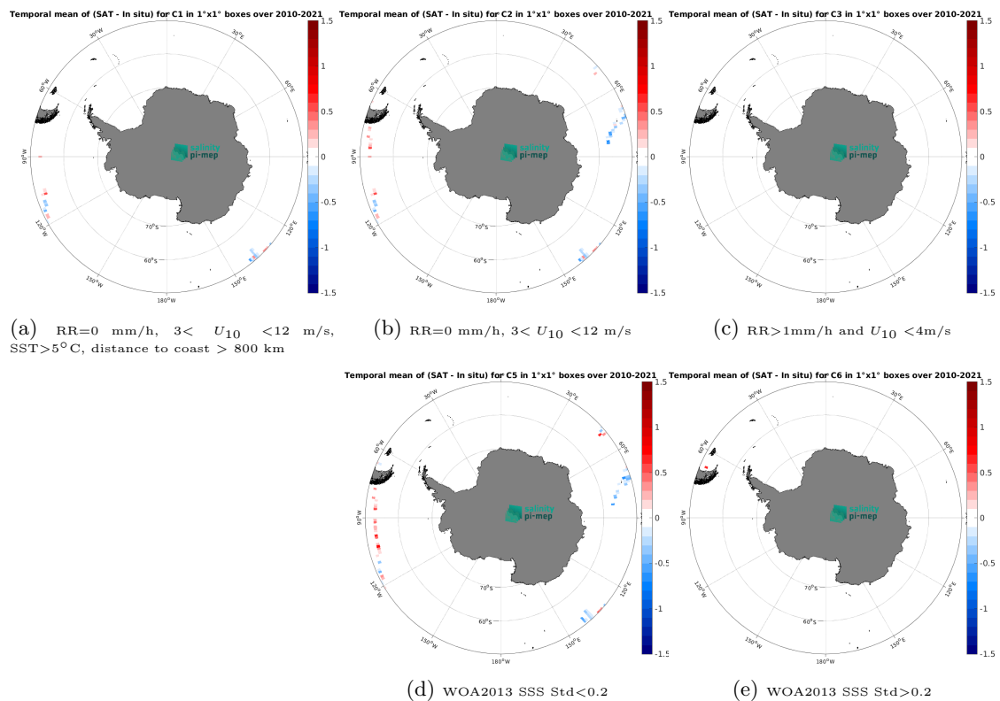
Figure 14: Temporal mean gridded over spatial boxes of size 1^\circ \times 1^\circ of \Delta\text{SSS} (SMOS SSS L3 v335 - Monthly - 25 km (CATDS-CPDC) - TSG (GOSUD-Research-vessel)) for 5 different subdatasets corresponding to:RR=0 mm/h, 3 < U_{10} < 12 m/s, SST>5°C, distance to coast > 800 km (a), RR=0 mm/h, 3 < U_{10} < 12 m/s (b), RR>1mm/h and U_{10} < 4 m/s (c), WOA2013 SSS Std<0.2 (d), WOA2013 SSS Std>0.2 (e).
