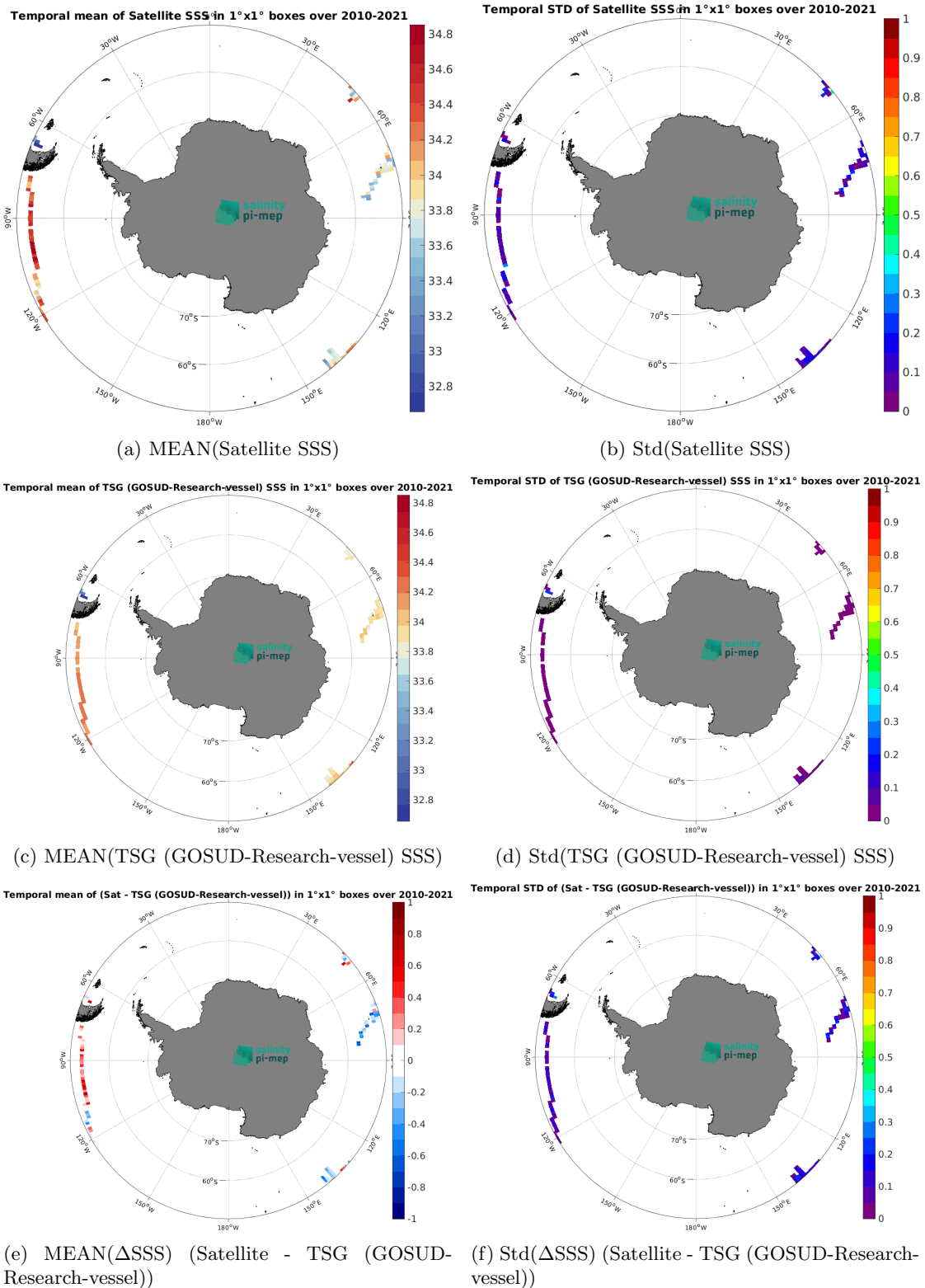
Figure 6: Temporal mean (left) and Std (right) of SSS from SMOS SSS L3 v335 - Monthly - 25 km (CATDS-CPDC) (top), TSG (GOSUD-Research-vessel) (middle), and of \Delta SSS (Satellite - TSG (GOSUD-Research-vessel)). Only match-17 pairs are used to generate these maps.
