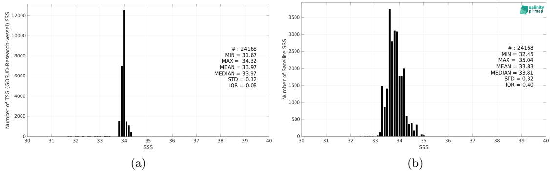
Figure 2: Histograms of SSS from TSG (GOSUD-Research-vessel) (a) and SMOS SSS L3 v335 - Monthly - 25 km (CATDS-CPDC) (b) considering all match-up pairs per bins of 0.1 over the Southern Ocean Pi-MEP region and for the full satellite product period.
