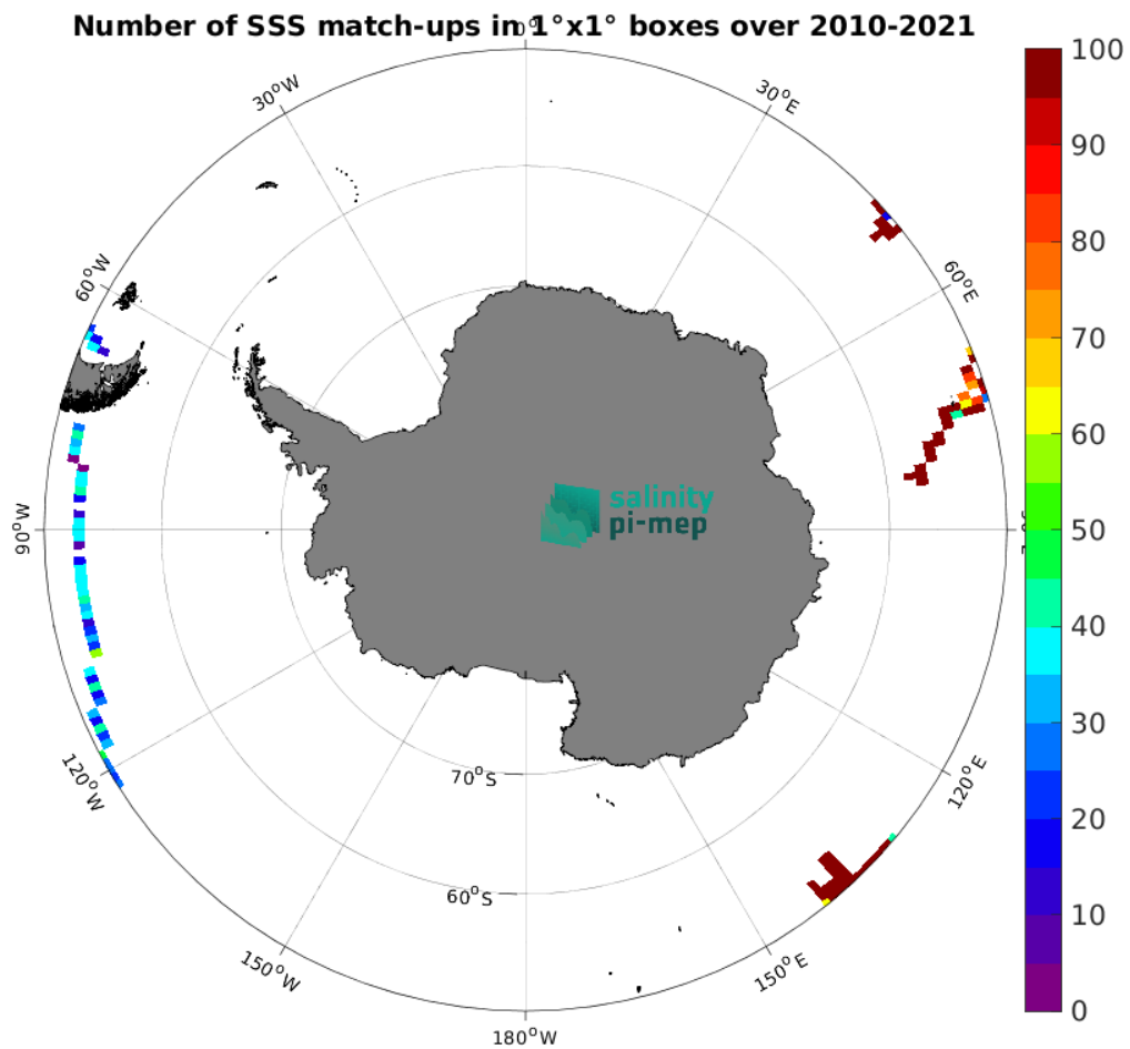
Figure 4: Number of SSS match-ups between TSG (GOSUD-Research-vessel) SSS and the SMOS SSS L3 v335 - Monthly - 25 km (CATDS-CPDC) SSS product for the Southern Ocean Pi-MEP region over 1^\circ \times 1^\circ boxes and for the full satellite product period.
