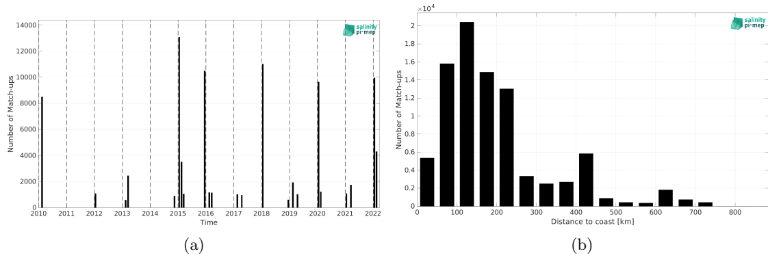
Figure 2: Number of match-ups between TSG (CSIC-UTM) and SMOS SSS L3 v335 - Monthly - 25 km (CATDS-CPDC) SSS as a function of time (a) and as function of the distance to coast (b) over the Southern Ocean Pi-MEP region and for the full satellite product period.
