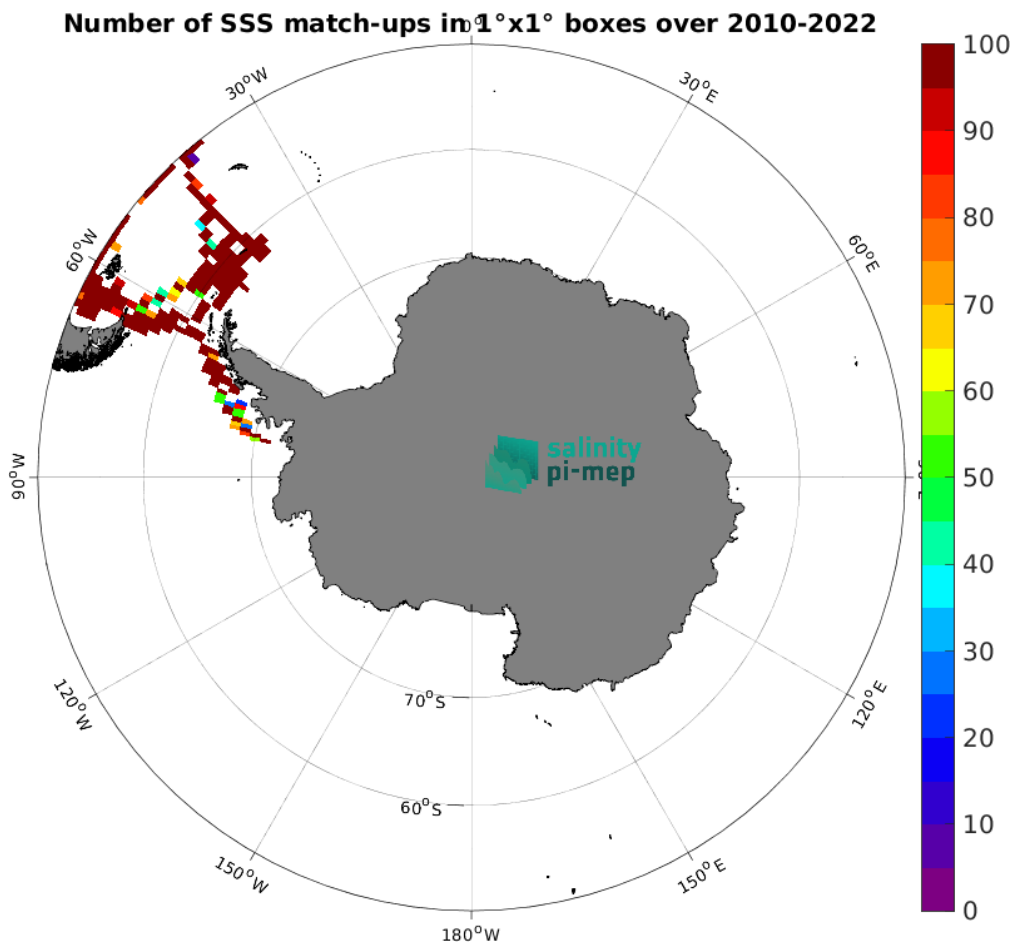
Figure 5: Number of SSS match-ups between TSG (CSIC-UTM) SSS and the SMOS SSS L3 v335 - Monthly - 25 km (CATDS-CPDC) SSS product for the Southern Ocean Pi-MEP region over 1^{\circ} \times 1^{\circ} boxes and for the full satellite product period.
