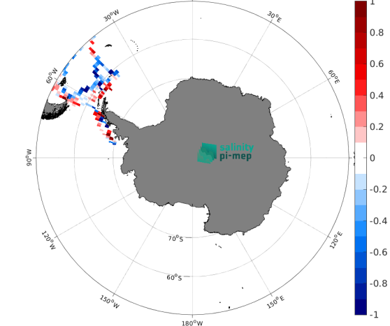
(e) MEAN( \Delta SSS) (Satellite - TSG (CSIC-UTM)) 17
