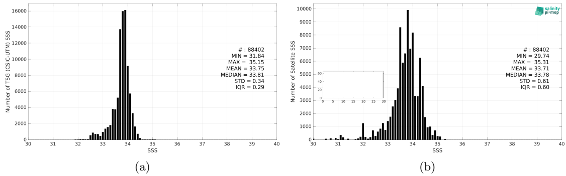
Figure 3: Histograms of SSS from TSG (CSIC-UTM) (a) and SMOS SSS L3 v335 - Monthly - 25 km (CATDS-CPDC) (b) considering all match-up pairs per bins of 0.1 over the Southern Ocean Pi-MEP region and for the full satellite product period.
