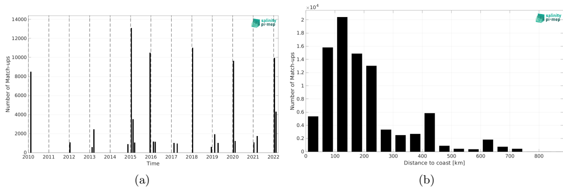
Figure 1: Number of match-ups between TSG (CSIC-UTM) and SMOS SSS L3 v335 - Monthly - 25 km (CATDS-CPDC) SSS as a function of time (a) and as function of the distance to coast (b) over the Southern Ocean Pi-MEP region and for the full satellite product period.
