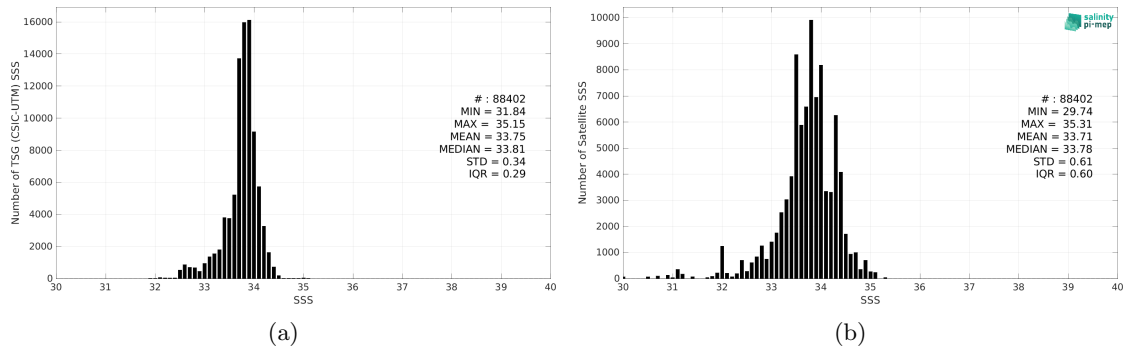
Figure 2: Histograms of SSS from TSG (CSIC-UTM) (a) and SMOS SSS L3 v335 - Monthly - 25 km (CATDS-CPDC) (b) considering all match-up pairs per bins of 0.1 over the Southern Ocean Pi-MEP region and for the full satellite product period.
