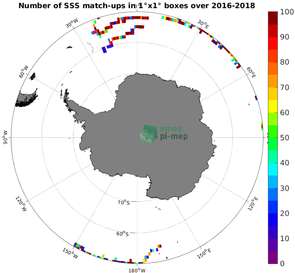
Figure 3: Number of SSS match-ups between Surface drifters SSS and the SMOS SSS L3 v335 - Monthly - 25 km (CATDS-CPDC) SSS product for the Southern Ocean Pi-MEP region over 1^\circ \times 1^\circ boxes and for the full satellite product period.
