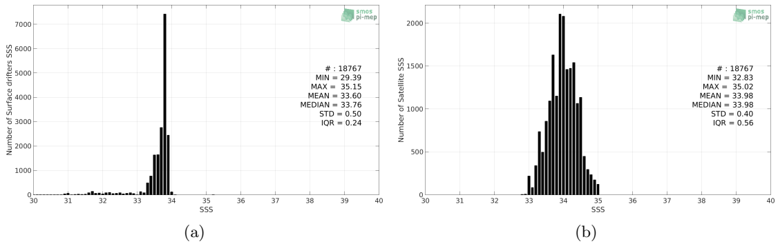
Figure 2: Histograms of SSS from Surface drifters (a) and SMOS SSS L3 v335 - Monthly - 25 km (CATDS-CPDC) (b) considering all match-up pairs per bins of 0.1 over the Southern Ocean Pi-MEP region and for the full satellite product period.
