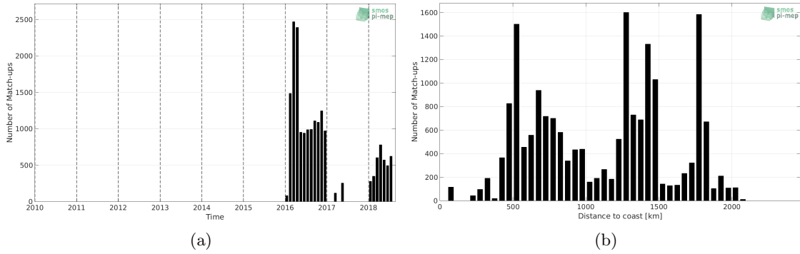
Figure 1: Number of match-ups between Surface drifters and SMOS SSS L3 v335 - Monthly - 25 km (CATDS-CPDC) SSS as a function of time (a) and as function of the distance to coast (b) over the Southern Ocean Pi-MEP region and for the full satellite product period.
