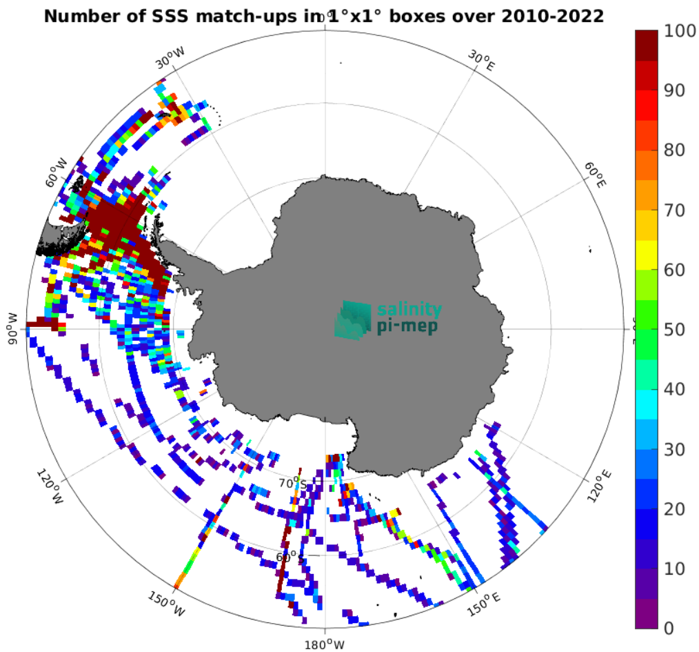
Figure 4: Number of SSS match-ups between TSG (SAMOS) SSS and the SMOS SSS L3 v335 - 10 Days - 25 km (CATDS-CPDC) SSS product for the Southern Ocean Pi-MEP region over 1^\circ \times 1^\circ boxes and for the full satellite product period.
