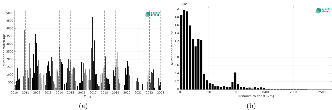
Figure 1: Number of match-ups between TSG (SAMOS) and SMOS SSS L3 v335 - 10 Days - 25 km (CATDS-CPDC) SSS as a function of time (a) and as function of the distance to coast (b) over the Southern Ocean Pi-MEP region and for the full satellite product period.
