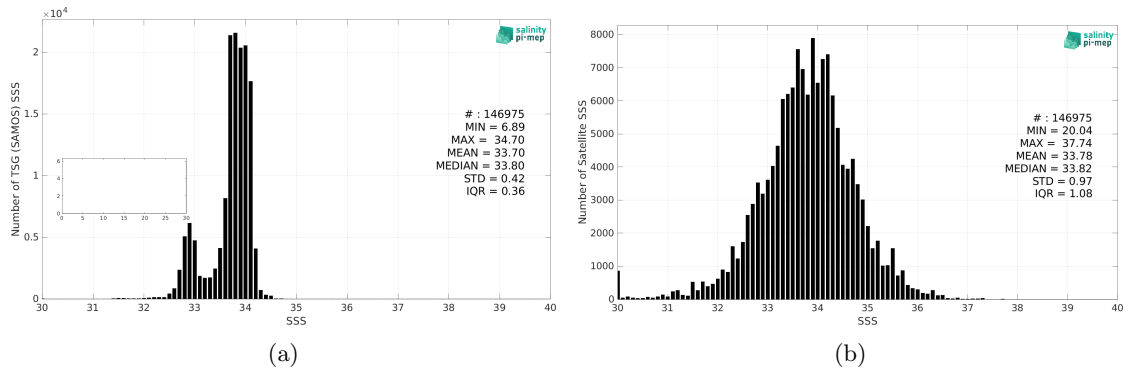
Figure 2: Histograms of SSS from TSG (SAMOS) (a) and SMOS SSS L3 v335 - 10 Days - 25 km (CATDS-CPDC) (b) considering all match-up pairs per bins of 0.1 over the Southern Ocean Pi-MEP region and for the full satellite product period.
