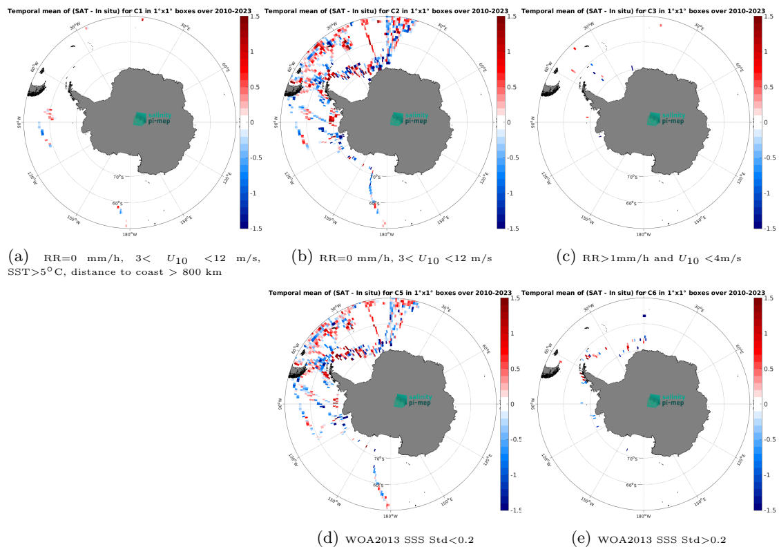
Figure 14: Temporal mean gridded over spatial boxes of size 1^\circ \times 1^\circ of \Delta SSS (SMOS SSS L3 v335 - 10 Days - 25 km (CATDS-CPDC) - TSG (Polarstern)) for 5 different subdatasets corresponding to: RR=0 mm/h, 3 < U_{10} < 12 m/s, SST > 5^\circ\text{C} , distance to coast > 800 km (a), RR=0 mm/h, 3 < U_{10} < 12 m/s (b), RR > 1 mm/h and U_{10} < 4 m/s (c), WOA2013 SSS Std < 0.2 (d), WOA2013 SSS Std > 0.2 (e).
