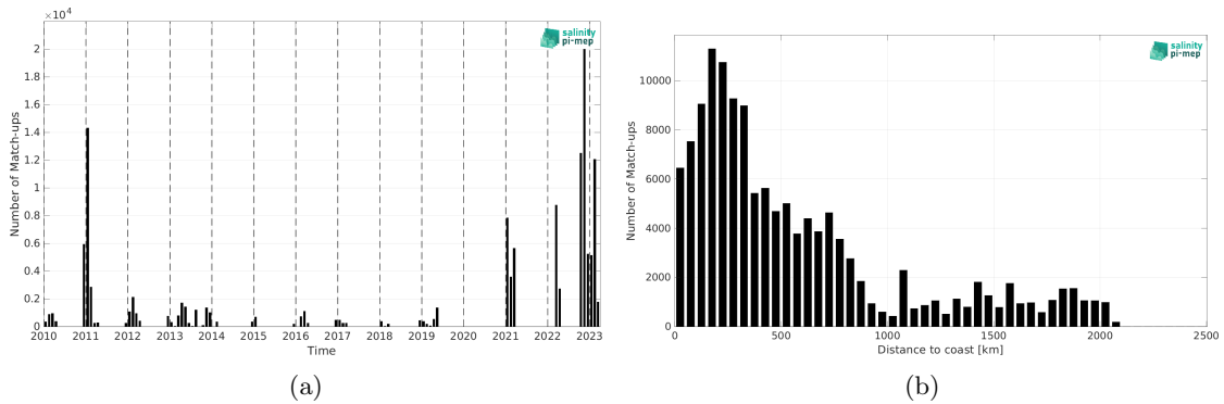
Figure 2: Number of match-ups between TSG (Polarstern) and SMOS SSS L3 v335 - 10 Days - 25 km (CATDS-CPDC) SSS as a function of time (a) and as function of the distance to coast (b) over the Southern Ocean Pi-MEP region and for the full satellite product period.
