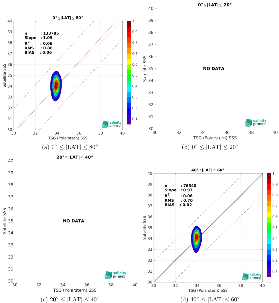
Figure 10: Contour maps of the concentration of SMOS SSS L3 v335 - 10 Days - 25 km (CATDS-CPDC) SSS (y-axis) versus TSG (Polarstern) SSS (x-axis) at match-up pairs for different latitude bands. For each plot, the red line shows x=y . The black thin and dashed lines indicate a linear fit through the data cloud and the \pm 95\% confidence levels, respectively. The number match-up pairs n , the slope and R^2 coefficient of the linear fit, the root mean square (RMS) and the mean bias between satellite and in situ data are indicated for each latitude band in each plots.
