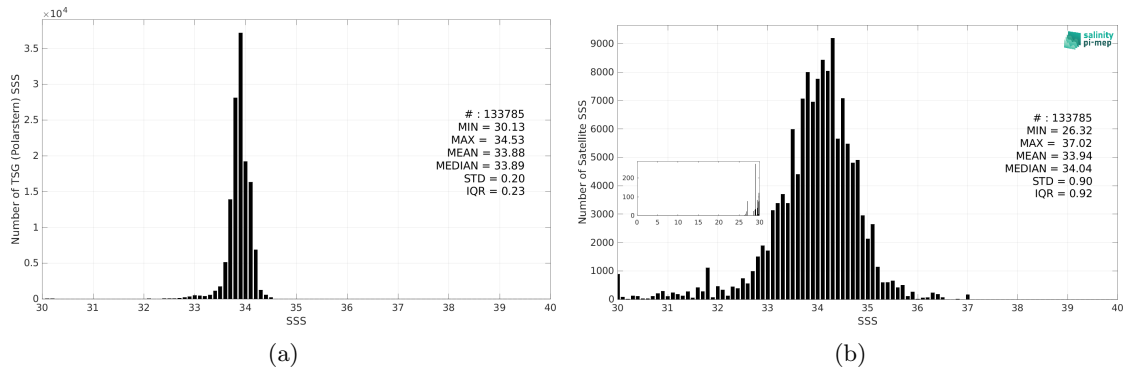
Figure 3: Histograms of SSS from TSG (Polarstern) (a) and SMOS SSS L3 v335 - 10 Days - 25 km (CATDS-CPDC) (b) considering all match-up pairs per bins of 0.1 over the Southern Ocean Pi-MEP region and for the full satellite product period.
