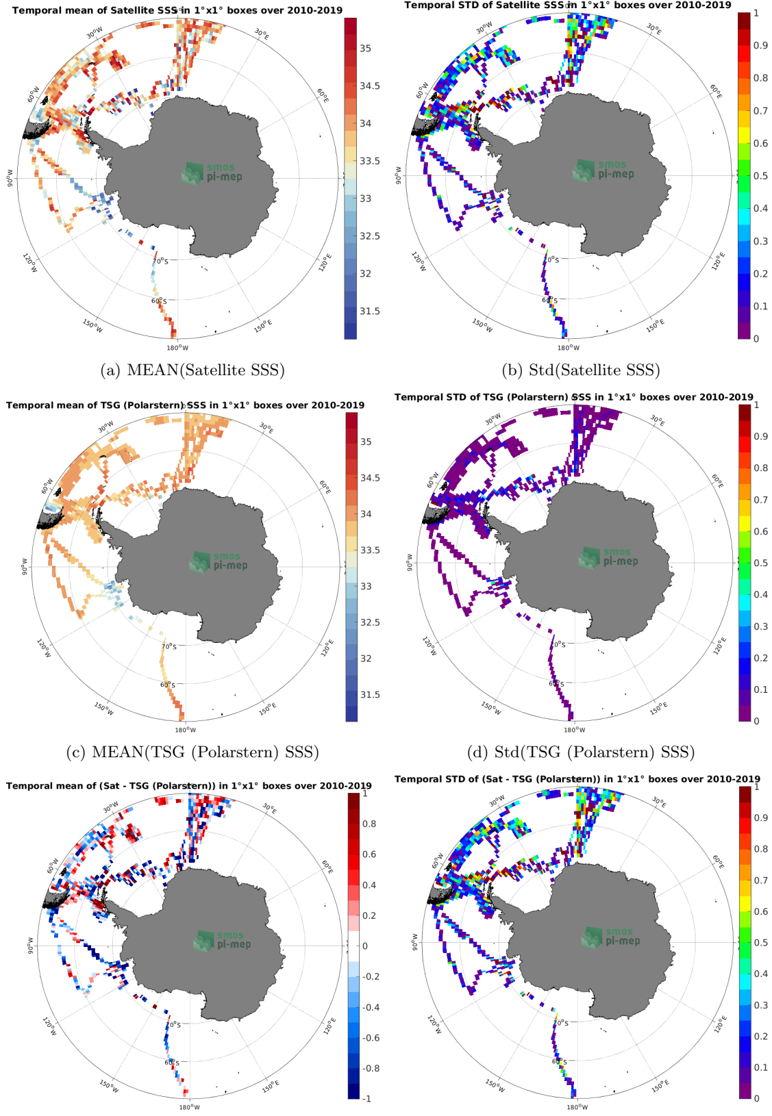
(e) MEAN( \Delta SSS) (Satellite - TSG (Polarstern)) 17 (f) Std( \Delta SSS) (Satellite - TSG (Polarstern)) Figure 6: Temporal mean (left) and Std (right) of SSS from SMOS SSS L3 v335 - 10 Days - 25 km (CATDS-CPDC) (top), TSG (Polarstern) (middle), and of \Delta SSS (Satellite - TSG (Polarstern)). Only match-up pairs are used to generate these maps.
