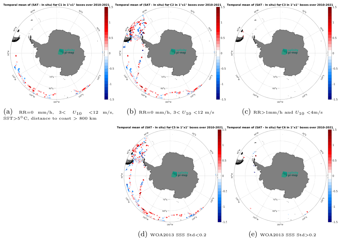
Figure 14: Temporal mean gridded over spatial boxes of size 1^\circ \times 1^\circ of \Delta\text{SSS} (SMOS SSS L3 v335 - 10 Days - 25 km (CATDS-CPDC) - TSG (GOSUD-Sailing-ship)) for 5 different subdatasets corresponding to:RR=0 mm/h, 3 < U_{10} < 12 m/s, SST>5°C, distance to coast > 800 km (a), RR=0 mm/h, 3 < U_{10} < 12 m/s (b), RR>1mm/h and U_{10} < 4 m/s (c), WOA2013 SSS Std<0.2 (d), WOA2013 SSS Std>0.2 (e).
