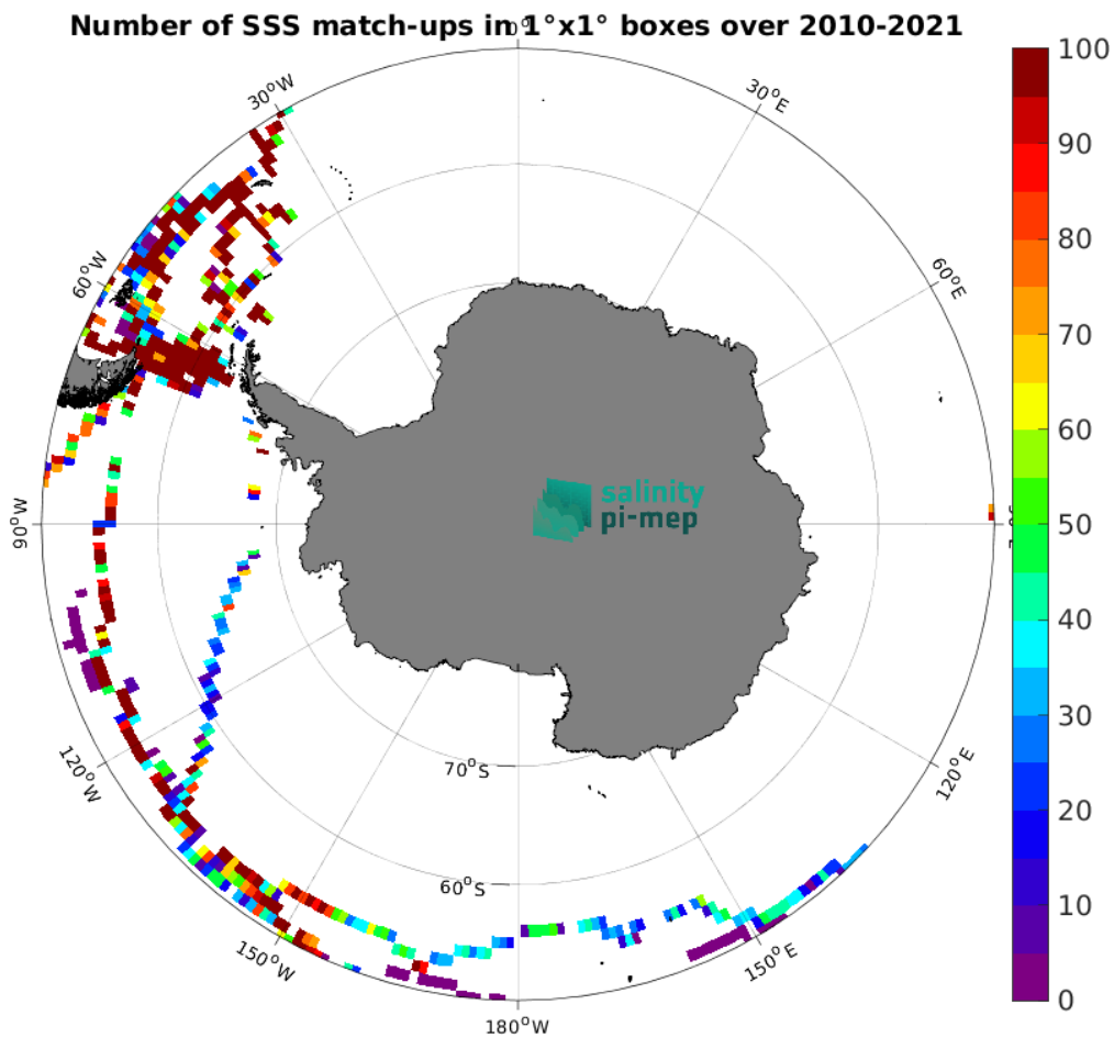
Figure 5: Number of SSS match-ups between TSG (GOSUD-Sailing-ship) SSS and the SMOS SSS L3 v335 - 10 Days - 25 km (CATDS-CPDC) SSS product for the Southern Ocean Pi-MEP region over 1^{\circ} \times 1^{\circ} boxes and for the full satellite product period.
