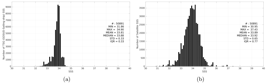
Figure 3: Histograms of SSS from TSG (GOSUD-Sailing-ship) (a) and SMOS SSS L3 v335 - 10 Days - 25 km (CATDS-CPDC) (b) considering all match-up pairs per bins of 0.1 over the Southern Ocean Pi-MEP region and for the full satellite product period.
