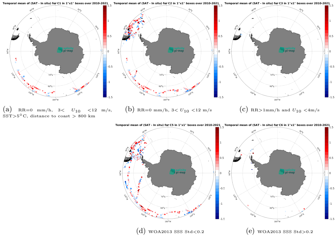
Figure 12: Temporal mean gridded over spatial boxes of size 1^{\circ} \times 1^{\circ} of \Delta SSS (SMOS SSS L3 v335 - 10 Days - 25 km (CATDS-CPDC) - TSG (GOSUD-Sailing-ship)) for 5 different subdatasets corresponding to:RR=0 mm/h, 3 < U_{10} < 12 m/s, SST>5°C, distance to coast > 800 km (a), RR=0 mm/h, 3 < U_{10} < 12 m/s (b), RR>1mm/h and U_{10} < 4 m/s (c), WOA2013 SSS Std<0.2 (d), WOA2013 SSS Std>0.2 (e).
