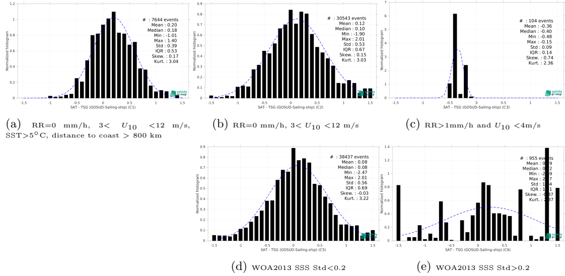
Figure 13: Normalized histogram of \Delta\text{SSS} (SMOS SSS L3 v335 - 10 Days - 25 km (CATDS-CPDC) - TSG (GOSUD-Sailing-ship)) for 5 different subdatasets corresponding to: RR=0 mm/h, 3 < U_{10} < 12 m/s, SST>5°C, distance to coast > 800 km (a), RR=0 mm/h, 3 < U_{10} < 12 m/s (b), RR>1mm/h and U_{10} < 4 m/s (c), WOA2013 SSS Std<0.2 (d), WOA2013 SSS Std>0.2 (e).
