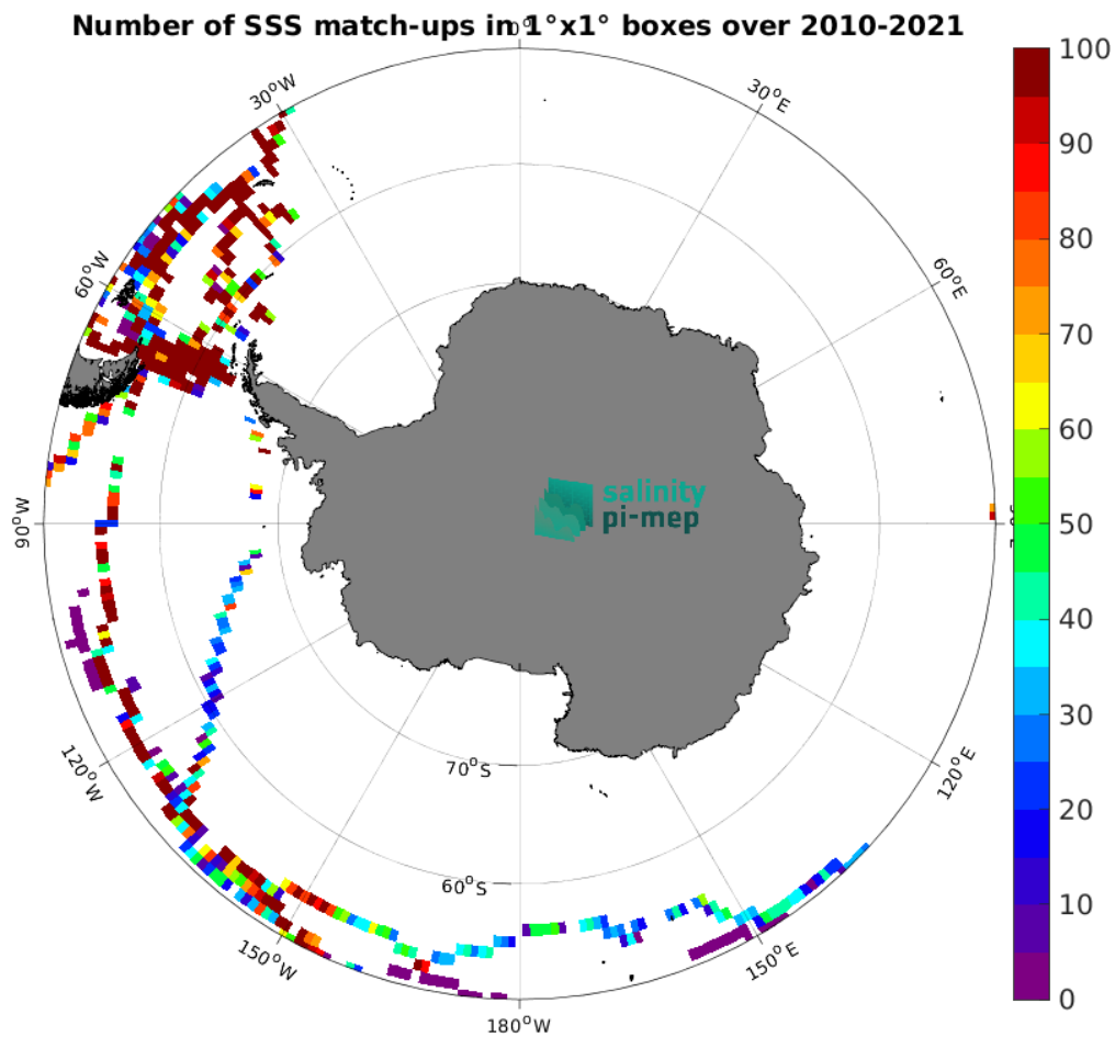
Figure 4: Number of SSS match-ups between TSG (GOSUD-Sailing-ship) SSS and the SMOS SSS L3 v335 - 10 Days - 25 km (CATDS-CPDC) SSS product for the Southern Ocean Pi-MEP region over 1^{\circ} \times 1^{\circ} boxes and for the full satellite product period.
