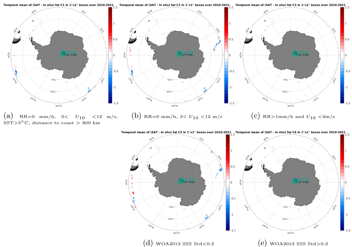
Figure 14: Temporal mean gridded over spatial boxes of size 1^\circ \times 1^\circ of \Delta\text{SSS} (SMOS SSS L3 v335 - 10 Days - 25 km (CATDS-CPDC) - TSG (GOSUD-Research-vessel)) for 5 different subdatasets corresponding to:RR=0 mm/h, 3 < U_{10} < 12 m/s, SST >5^\circ\text{C} , distance to coast > 800 km (a), RR=0 mm/h, 3 < U_{10} < 12 m/s (b), RR >1 mm/h and U_{10} < 4 m/s (c), WOA2013 SSS Std <0.2 (d), WOA2013 SSS Std >0.2 (e).
