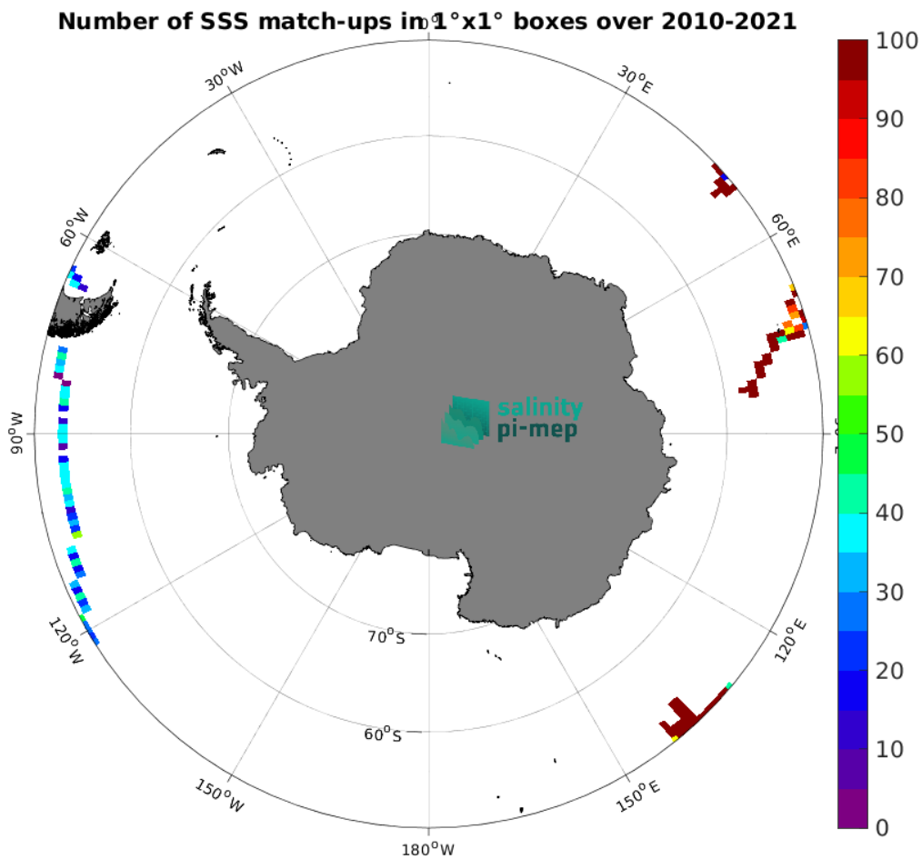
Figure 5: Number of SSS match-ups between TSG (GOSUD-Research-vessel) SSS and the SMOS SSS L3 v335 - 10 Days - 25 km (CATDS-CPDC) SSS product for the Southern Ocean Pi-MEP region over 1^\circ \times 1^\circ boxes and for the full satellite product period.
