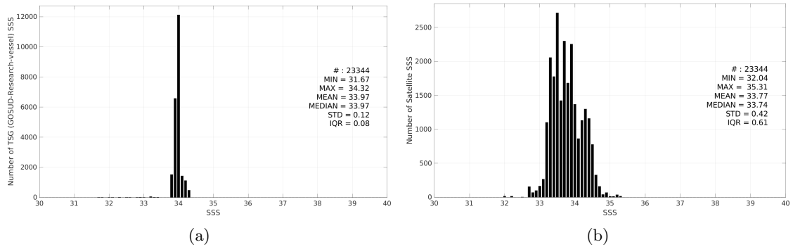
Figure 3: Histograms of SSS from TSG (GOSUD-Research-vessel) (a) and SMOS SSS L3 v335 - 10 Days - 25 km (CATDS-CPDC) (b) considering all match-up pairs per bins of 0.1 over the Southern Ocean Pi-MEP region and for the full satellite product period.
