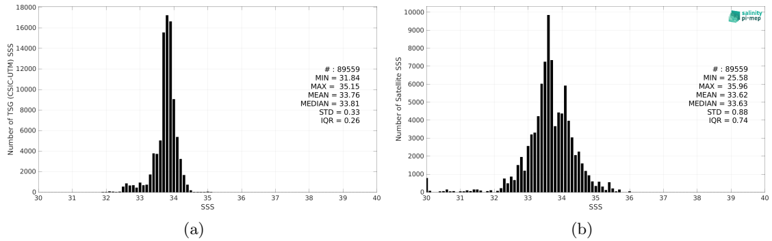
Figure 2: Histograms of SSS from TSG (CSIC-UTM) (a) and SMOS SSS L3 v335 - 10 Days - 25 km (CATDS-CPDC) (b) considering all match-up pairs per bins of 0.1 over the Southern Ocean Pi-MEP region and for the full satellite product period.
