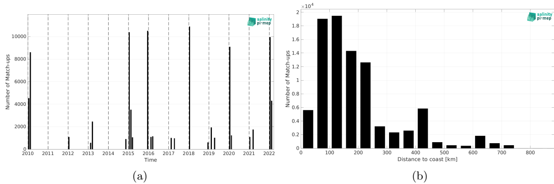
Figure 1: Number of match-ups between TSG (CSIC-UTM) and SMOS SSS L3 v335 - 10 Days - 25 km (CATDS-CPDC) SSS as a function of time (a) and as function of the distance to coast (b) over the Southern Ocean Pi-MEP region and for the full satellite product period.
