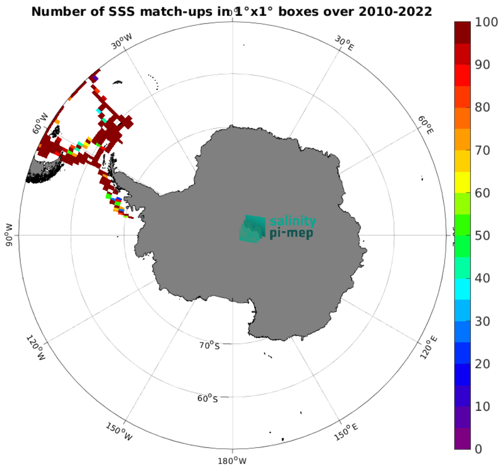
Figure 4: Number of SSS match-ups between TSG (CSIC-UTM) SSS and the SMOS SSS L3 v335 - 10 Days - 25 km (CATDS-CPDC) SSS product for the Southern Ocean Pi-MEP region over 1^{\circ} \times 1^{\circ} boxes and for the full satellite product period.
