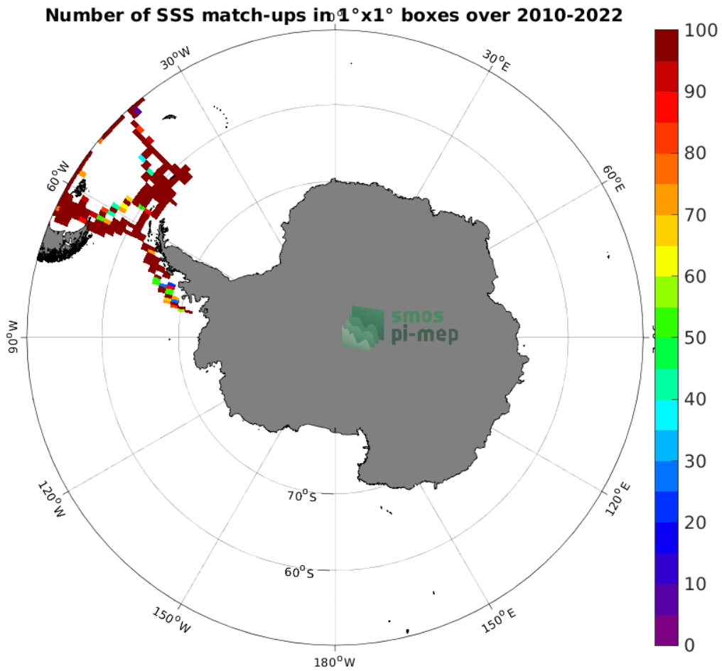
Figure 4: Number of SSS match-ups between TSG (CSIC-UTM) SSS and the SMOS SSS L3 v335 - 10 Days - 25 km (CATDS-CPDC) SSS product for the Southern Ocean Pi-MEP region over 1^\circ \times 1^\circ boxes and for the full satellite product period.
