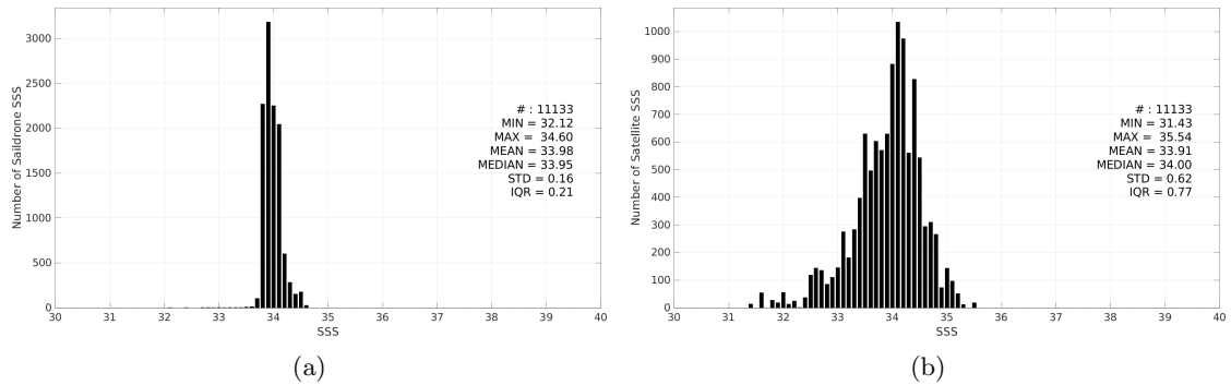
Figure 3: Histograms of SSS from Saildrone (a) and SMOS SSS L3 v335 - 10 Days - 25 km (CATDS-CPDC) (b) considering all match-up pairs per bins of 0.1 over the Southern Ocean Pi-MEP region and for the full satellite product period.
