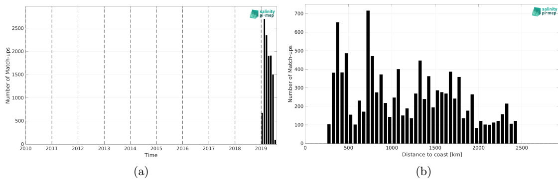
Figure 2: Number of match-ups between Saildrone and SMOS SSS L3 v335 - 10 Days - 25 km (CATDS-CPDC) SSS as a function of time (a) and as function of the distance to coast (b) over the Southern Ocean Pi-MEP region and for the full satellite product period.
