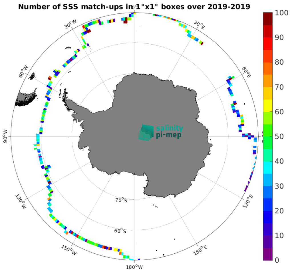
Figure 5: Number of SSS match-ups between Saildrone SSS and the SMOS SSS L3 v335 - 10 Days - 25 km (CATDS-CPDC) SSS product for the Southern Ocean Pi-MEP region over 1^\circ \times 1^\circ boxes and for the full satellite product period.
