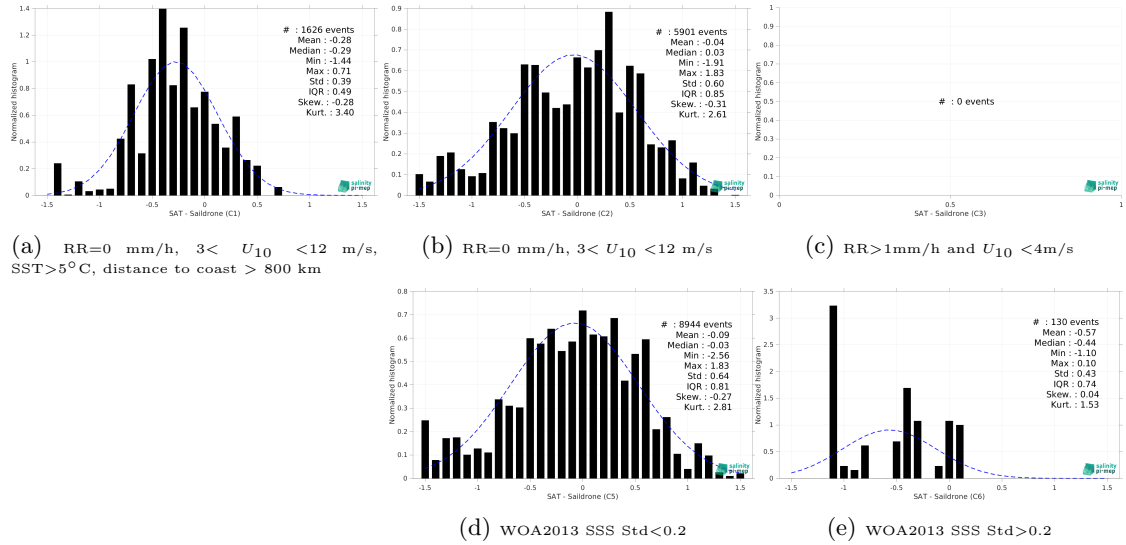
Figure 13: Normalized histogram of \Delta SSS (SMOS SSS L3 v335 - 10 Days - 25 km (CATDS-CPDC) - Saildrone) for 5 different subdatasets corresponding to: RR=0 mm/h, 3 < U_{10} < 12 m/s, SST > 5°C, distance to coast > 800 km (a), RR=0 mm/h, 3 < U_{10} < 12 m/s (b), RR > 1mm/h and U_{10} < 4 m/s (c), WOA2013 SSS Std < 0.2 (d), WOA2013 SSS Std > 0.2 (e).
