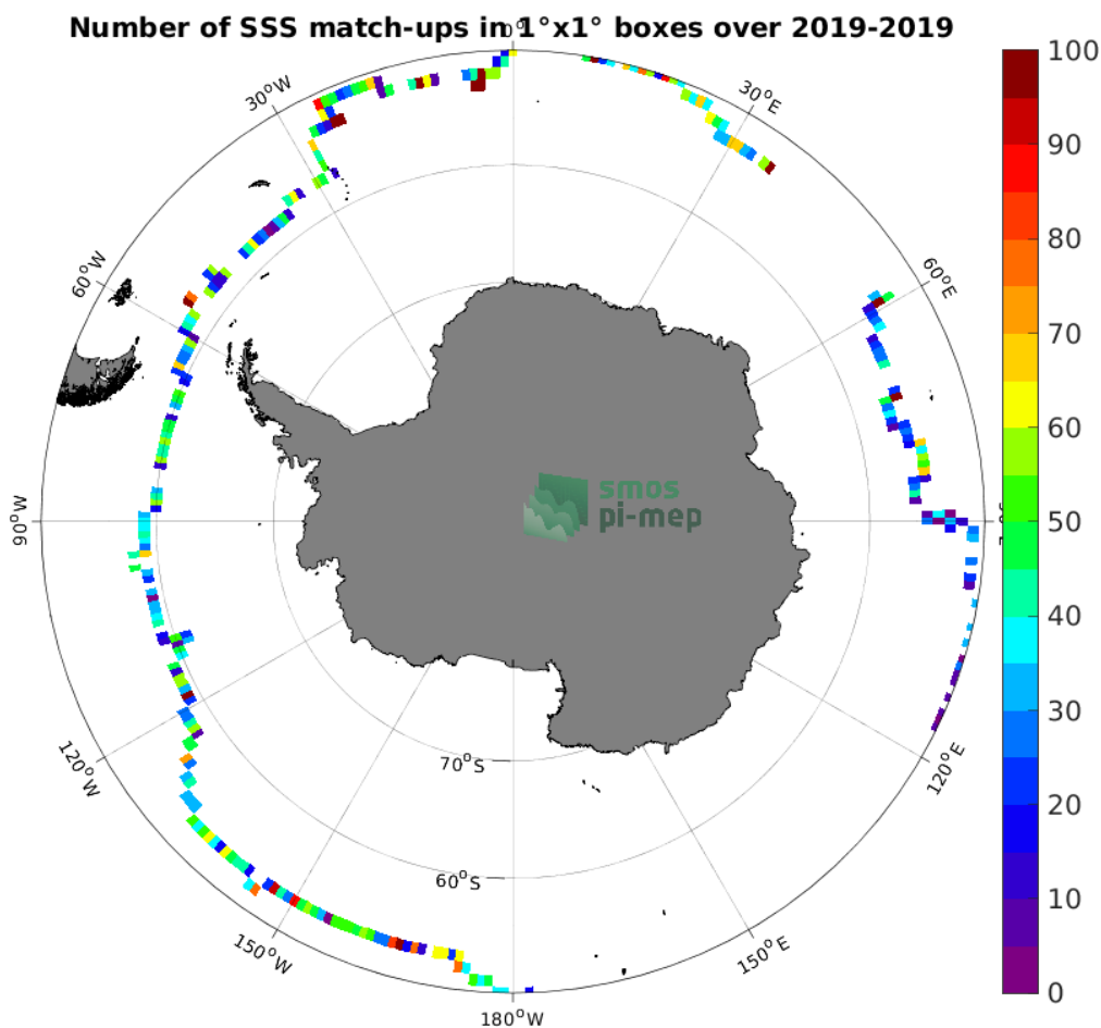
Figure 4: Number of SSS match-ups between Saildrone SSS and the SMOS SSS L3 v335 - 10 Days - 25 km (CATDS-CPDC) SSS product for the Southern Ocean Pi-MEP region over 1^\circ \times 1^\circ boxes and for the full satellite product period.
