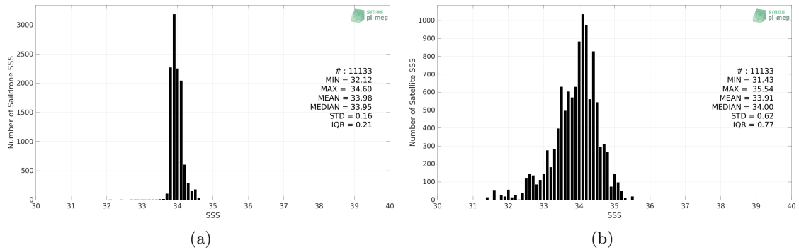
Figure 2: Histograms of SSS from Sairdrone (a) and SMOS SSS L3 v335 - 10 Days - 25 km (CATDS-CPDC) (b) considering all match-up pairs per bins of 0.1 over the Southern Ocean Pi-MEP region and for the full satellite product period.
