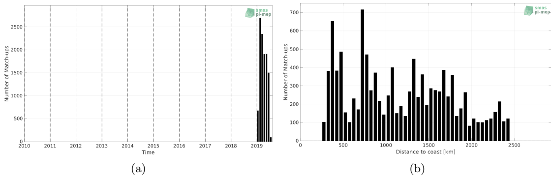
Figure 1: Number of match-ups between Saildrone and SMOS SSS L3 v335 - 10 Days - 25 km (CATDS-CPDC) SSS as a function of time (a) and as function of the distance to coast (b) over the Southern Ocean Pi-MEP region and for the full satellite product period.
